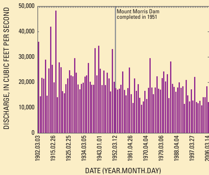
Figure 15. Peak flows on Genesee River at Rochester, N.Y., 1902–2007.
