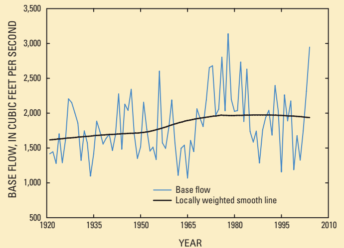
Figure 16. Annual mean base flows on Genesee River at Rochester, N.Y., 1920–2005.
