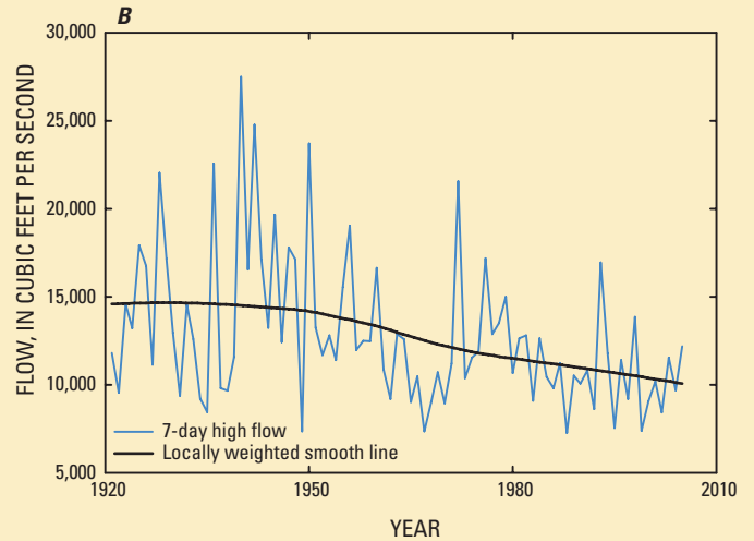
Figure 14. Seven-day (A) low and (B) high flows, Genesee River at Rochester, N.Y., 1920–2005.
