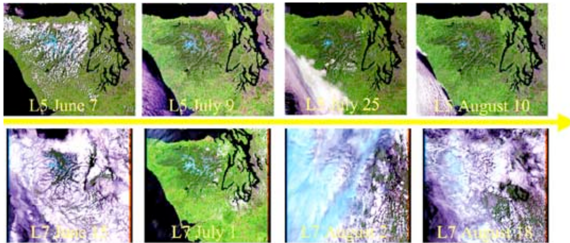
These images were taken by Landsats 5 and 7 from June through August 2001. They illustrate why regular repeated coverage by multiple satellites helps to ensure cloud-free images are acquired for users.
