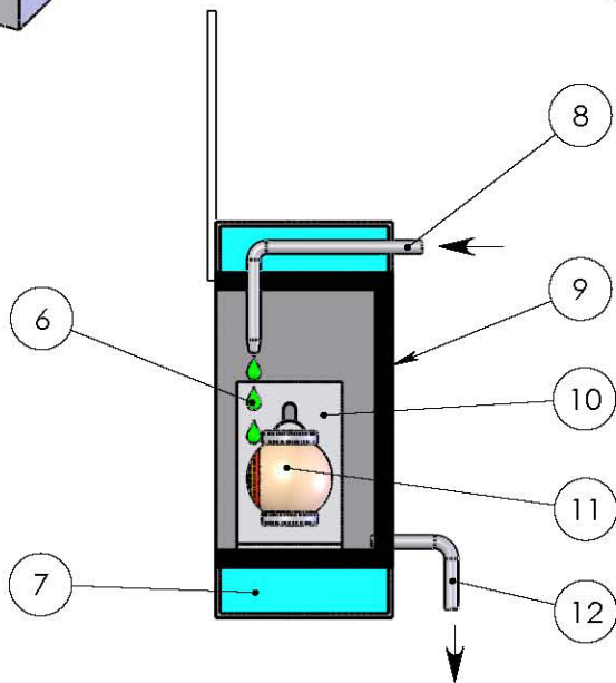
CROSS SECTION COMPARTMENT
