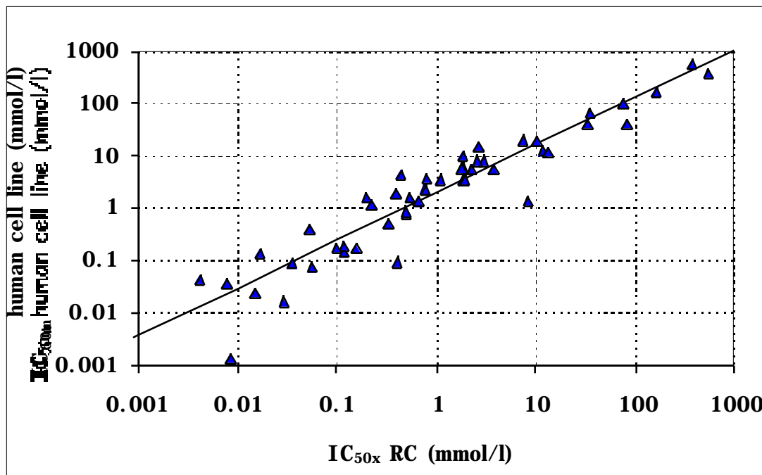
Figure A.4. Correlation between IC50x (averaged from various mammalian cell lines) of the RC and IC50m (from various human cell lines) is shown for the 50 MEIC chemicals. The linear correlation coefficient is high ( r = 0.95 ) and judged by an R^2 = 0.90 .
