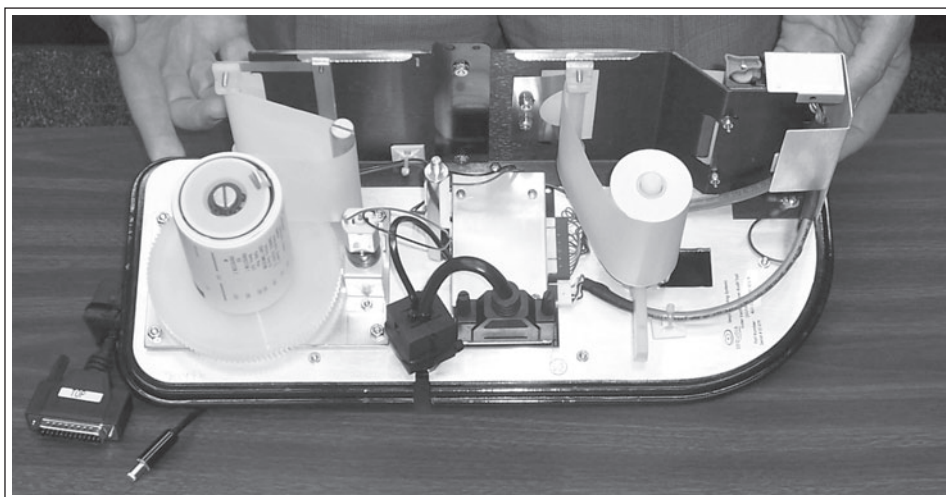
Figure 79: Example of an Assembly for Producing a Voter-Verifiable Paper Audit Trail for DRE Voting Equipment
