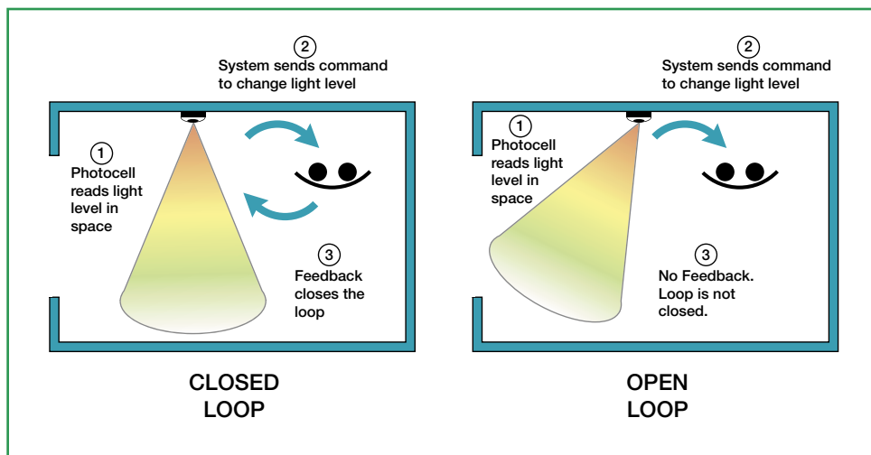
Figure 2. Closed and Open Loop Control Systems for Daylighting
