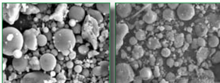
Figure 1. Bottom ash before (left) and after coating with ferric oxide
