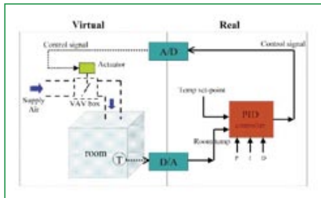
Figure 3. VAV control simulator example: hybrid software-hardware configuration
