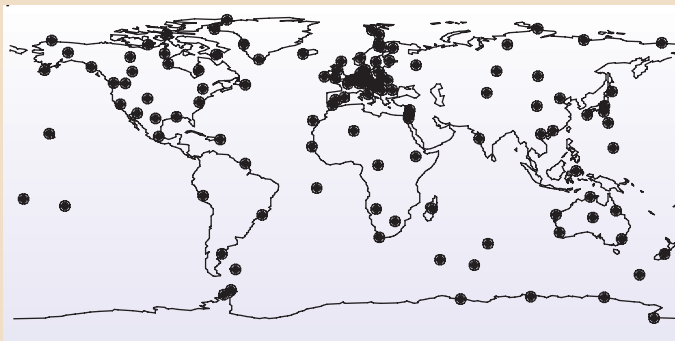
Figure 2. Worldwide distribution, as of 2006, of magnetic observatories that report one-minute-average digital data.
