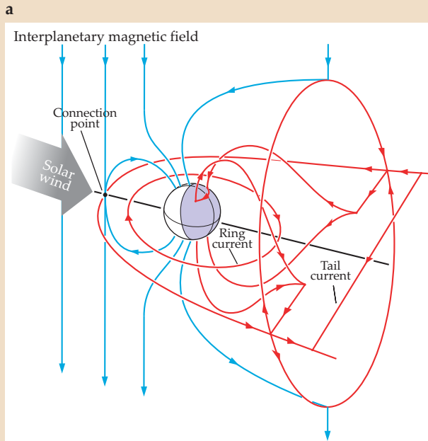
Figure 6. Earth's magnetosphere is shaped and controlled by the Sun. (a) Schematic representation of the magnetosphere. Blue lines represent magnetic fields, and red lines represent currents. Magnetic connection is shown on the day side of the magnetosphere, where a southward-pointing interplanetary field merges with a northward-pointing geomagnetic field. (b) Data from eight observatories show the disturbed horizontal intensity H during the Halloween magnetic storm of 28–31 October 2003. The magnetograms are arranged by longitude; red traces correspond to low-magnetic-latitude observatories and blue lines to observatories at high latitudes. The initial (I), main (M), and recovery (R) phases are discussed in the text. The circled anticorrelations between high- and low-latitude magnetograms are indicative of substorms.
