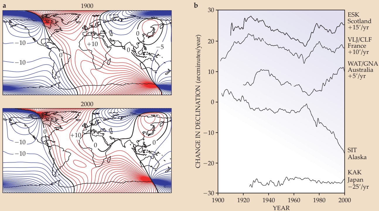
Figure 3. Magnetic declination changes over time. (a) Contour maps of declination D for the years 1900 and 2000 show significant differences over the century. Each contour line represents 5°; red is declination to the east and blue is to the west. (b) Data from five observatories show the yearly rate of change in declination. Note, in particular, the abrupt changes, or jerks, in the rate of secular variation, around 1970. For clarity of presentation, the data have been separated by the ordinate values listed on the right.
