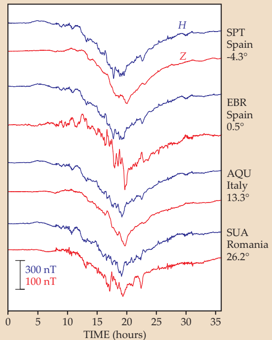
Figure 4. Magnetic-field variation reveals differences in subsurface electrical conductivity. Shown here are magnetograms taken on 20–21 November 2003 at European observatories of specified longitudes. Horizontal-intensity ( H , blue) variation is driven by a storm in the magnetosphere. Site-to-site differences in the downward ( Z , red) component are due to induced electric currents in the ocean and crust.
