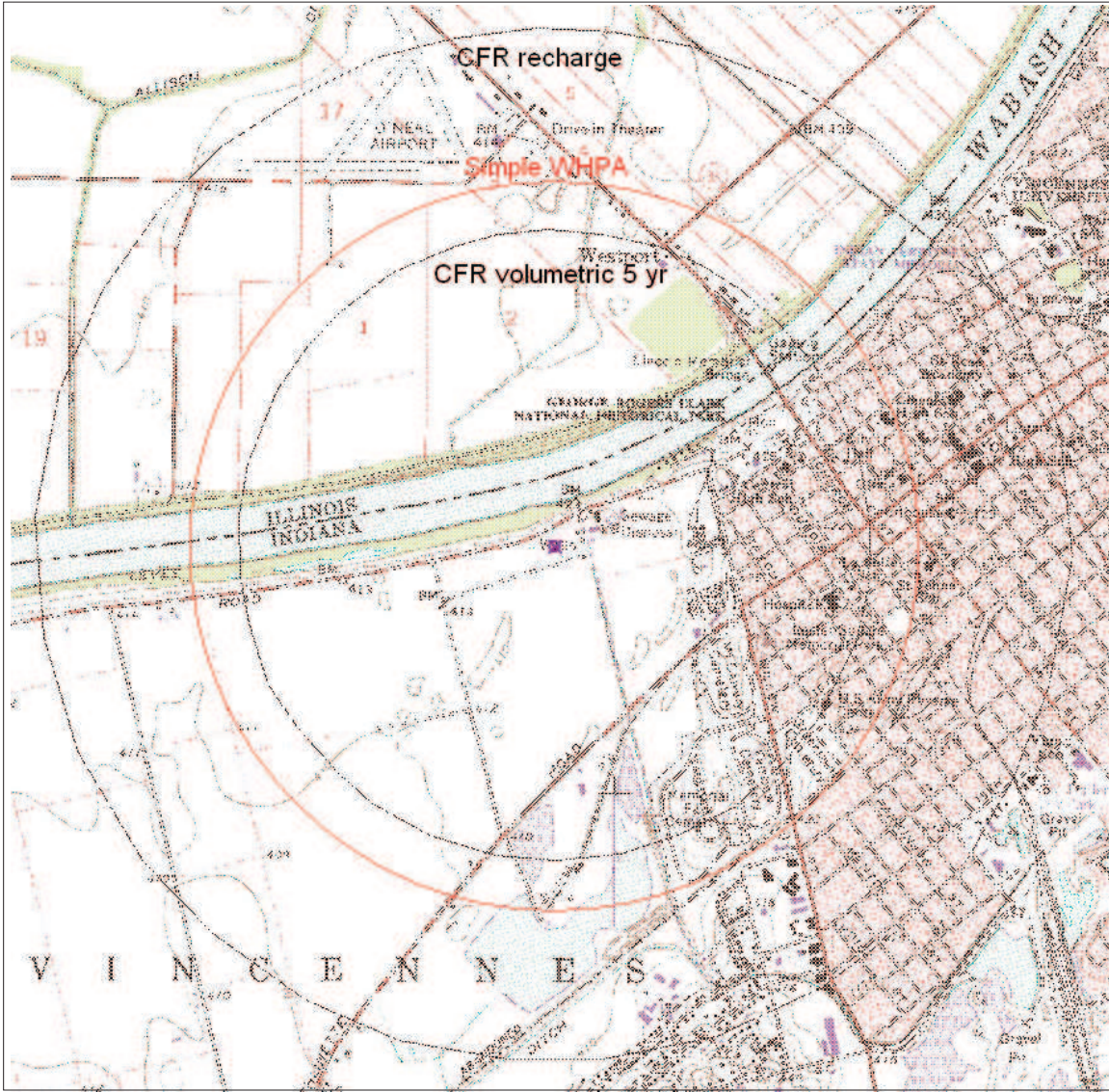
Figure 5.4: 5-yr Simple WHPA with no ambient flow compared to calculated fixed radius solutions using volumetric equation and recharge equation.
