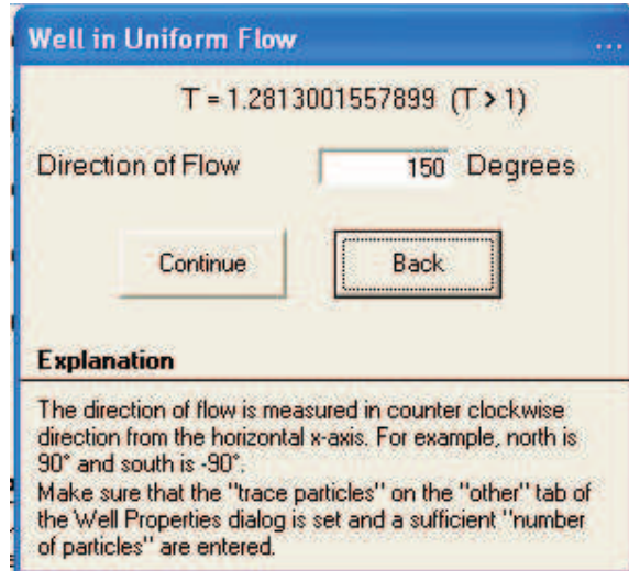
Figure 5.6: Dialog box simple well in uniform flow.
