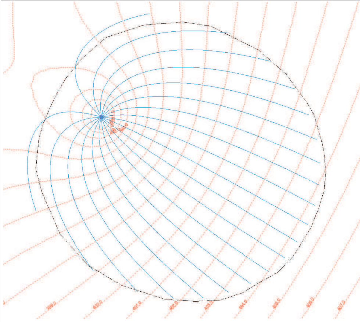
Figure 5.8: Simple WHPA including ambient flow compared to well in uniform flow.
