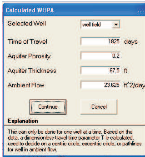
Figure 5.5: Dialog box calculated WHPA including ambient flow.
