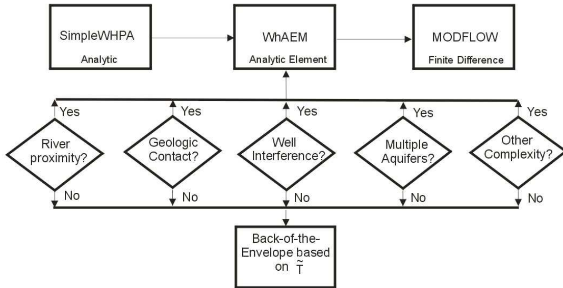
Figure 5.11: Decision tree for complexity of capture zone delineation method, after [Haitjema,2002].
