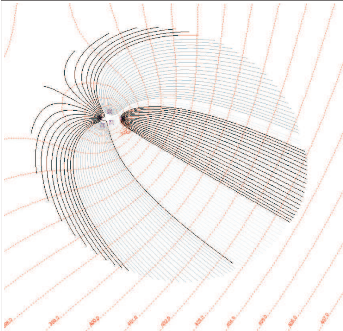
Figure 5.10: Simple WHPAs including multiple wells in ambient flow.
