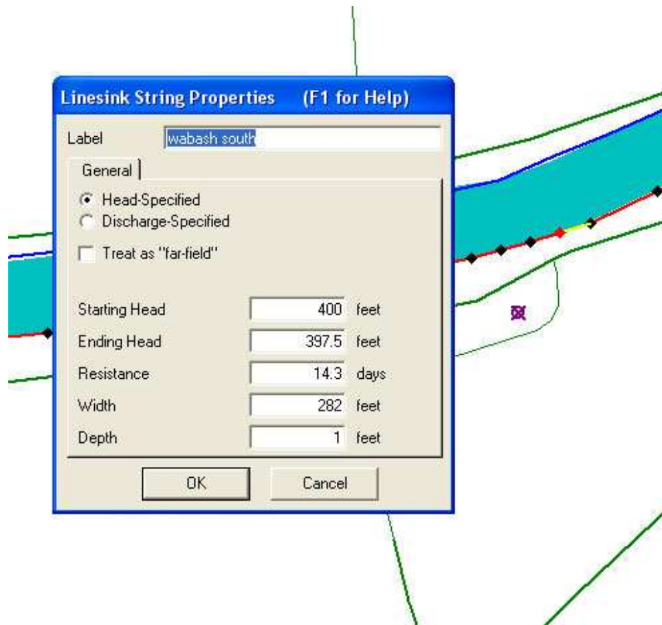
Figure 4.18: Dialog box for entry of resistance linesinks.
