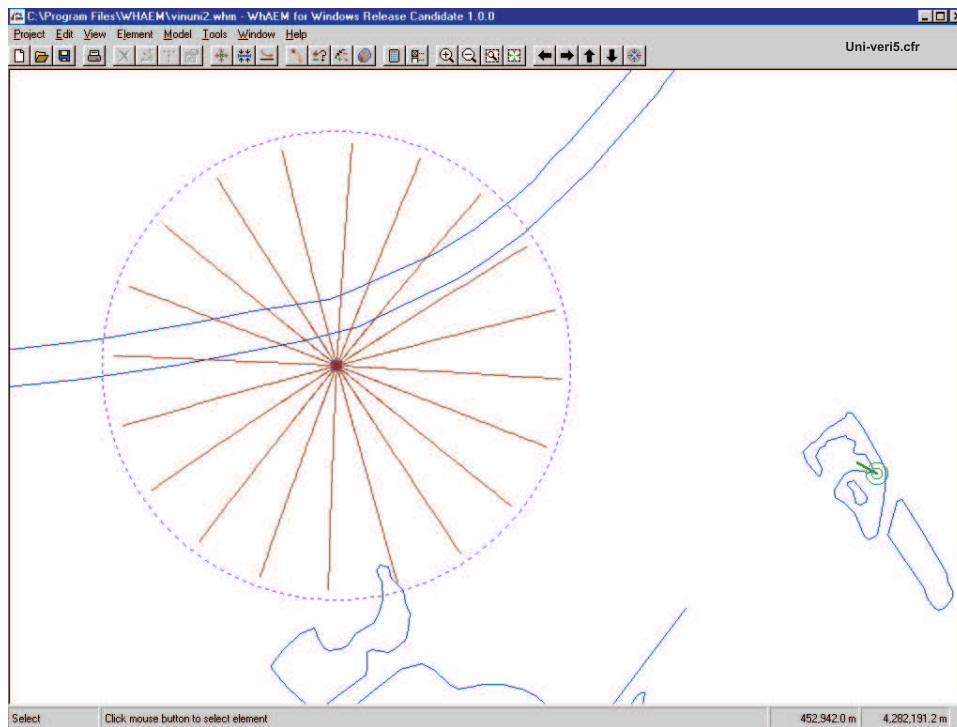
Figure 3.11: Capture zone based on 5 years residence time based on CFR volumetric and trachelines for well in uniform flow field (zero gradient).
