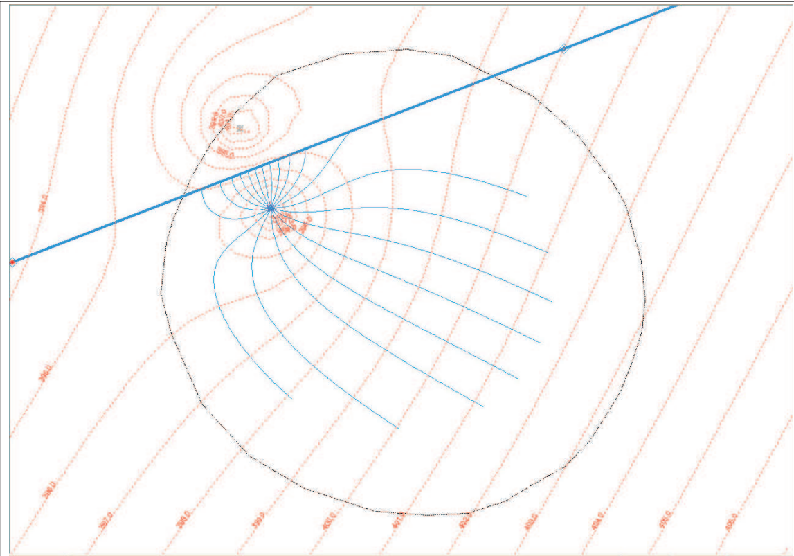
Figure 5.9: Simple WHPA including the influence of a stream boundary in comparison to capture zone for a well in uniform flow field.
