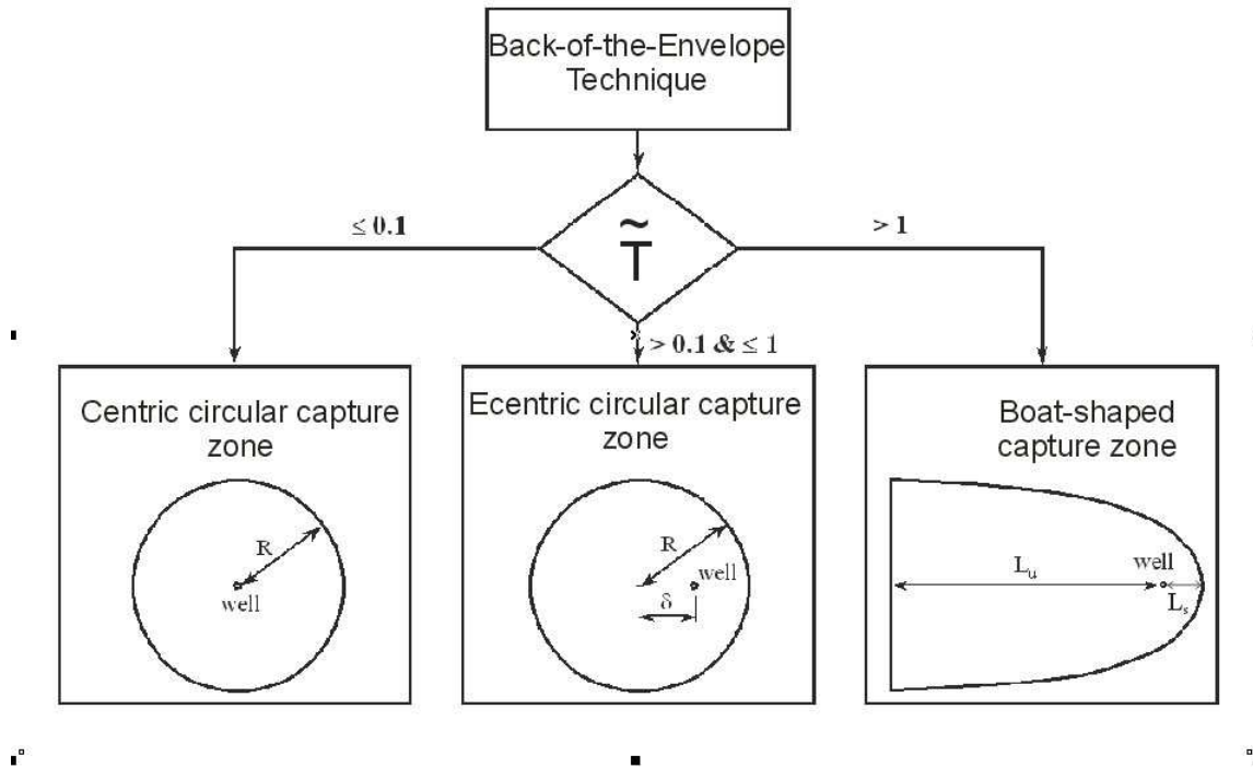
Figure 5.2: Simplified delineation techniques for a well pumping at rate Q , in an ambient flow field Q_o , with aquifer saturated thickness H and porosity n , and time of travel capture zones of time T , after [Haitjema,2002].
