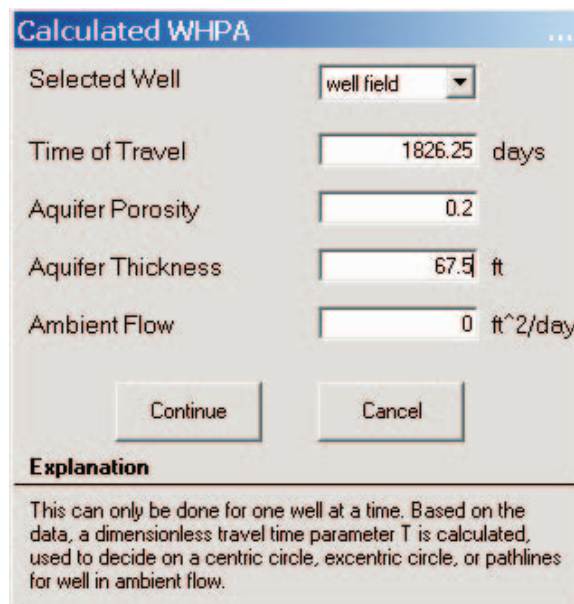
Figure 5.3: Dialog box for calculated WHPA.
