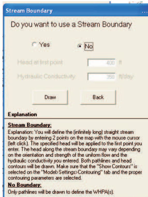
Figure 5.7: Dialog box simple stream boundary.
