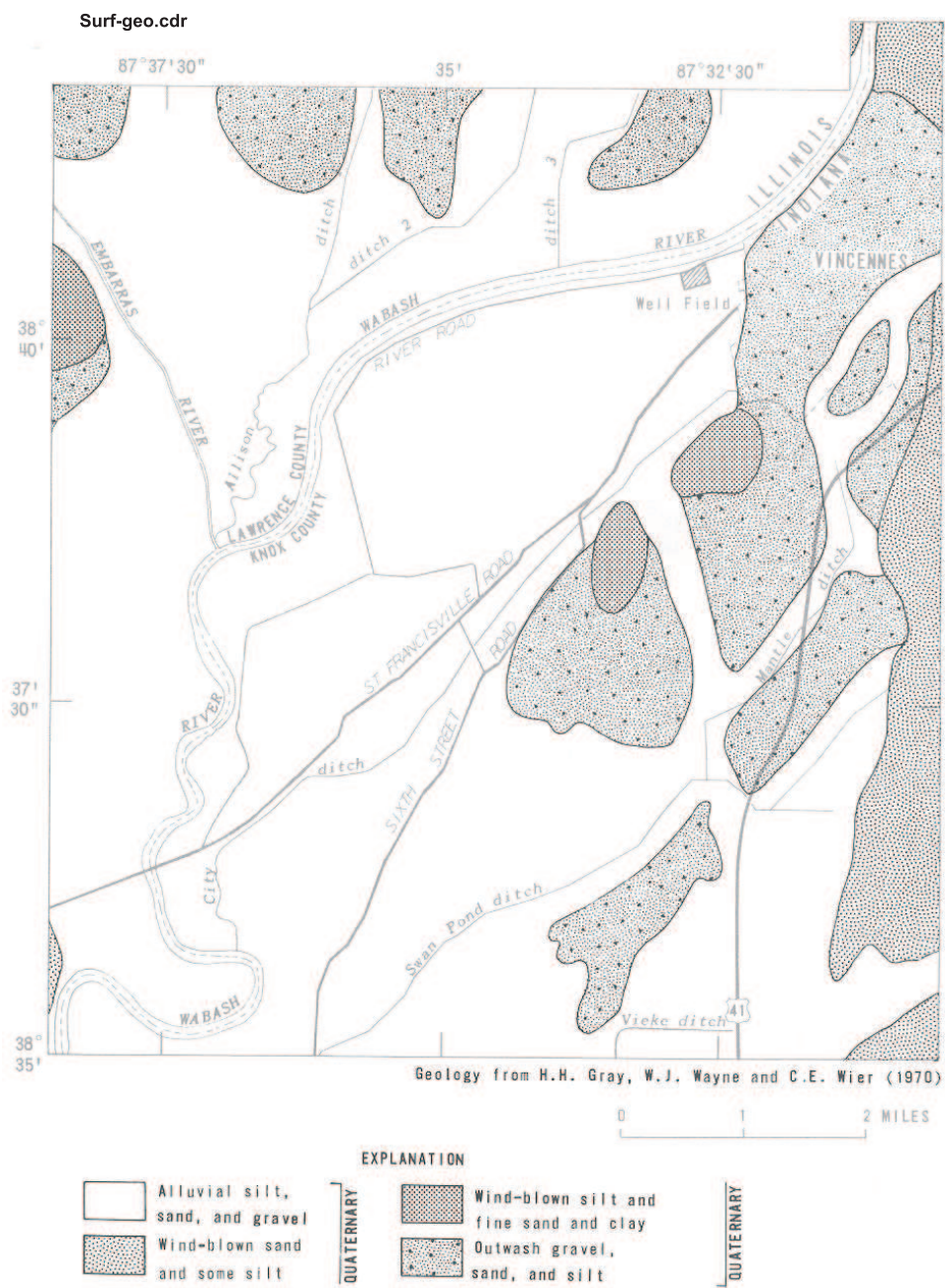
Figure 4.8: Surficial geology of the study region. [Shedlock,1980]
