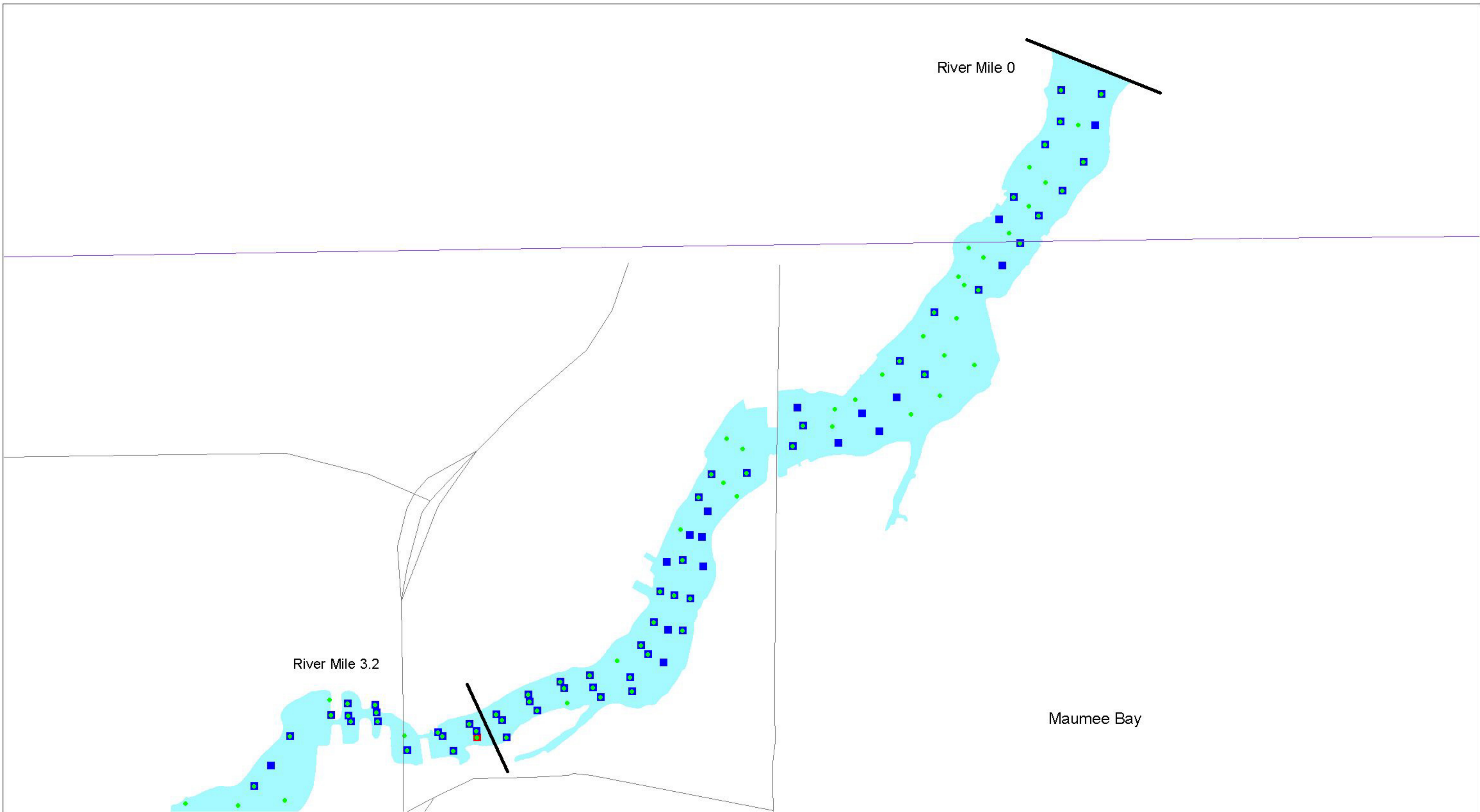
Figure D-6a : River Mile 0 - 3.2 Total PAH's in Sediment : 1998 Data Compared to Sediment Quality Guidelines (DiToro et al. 2000)
