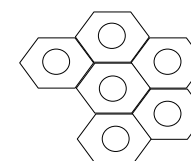
Benzo[ghi]perylene
