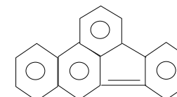
Benzo[b]fluoranthene
