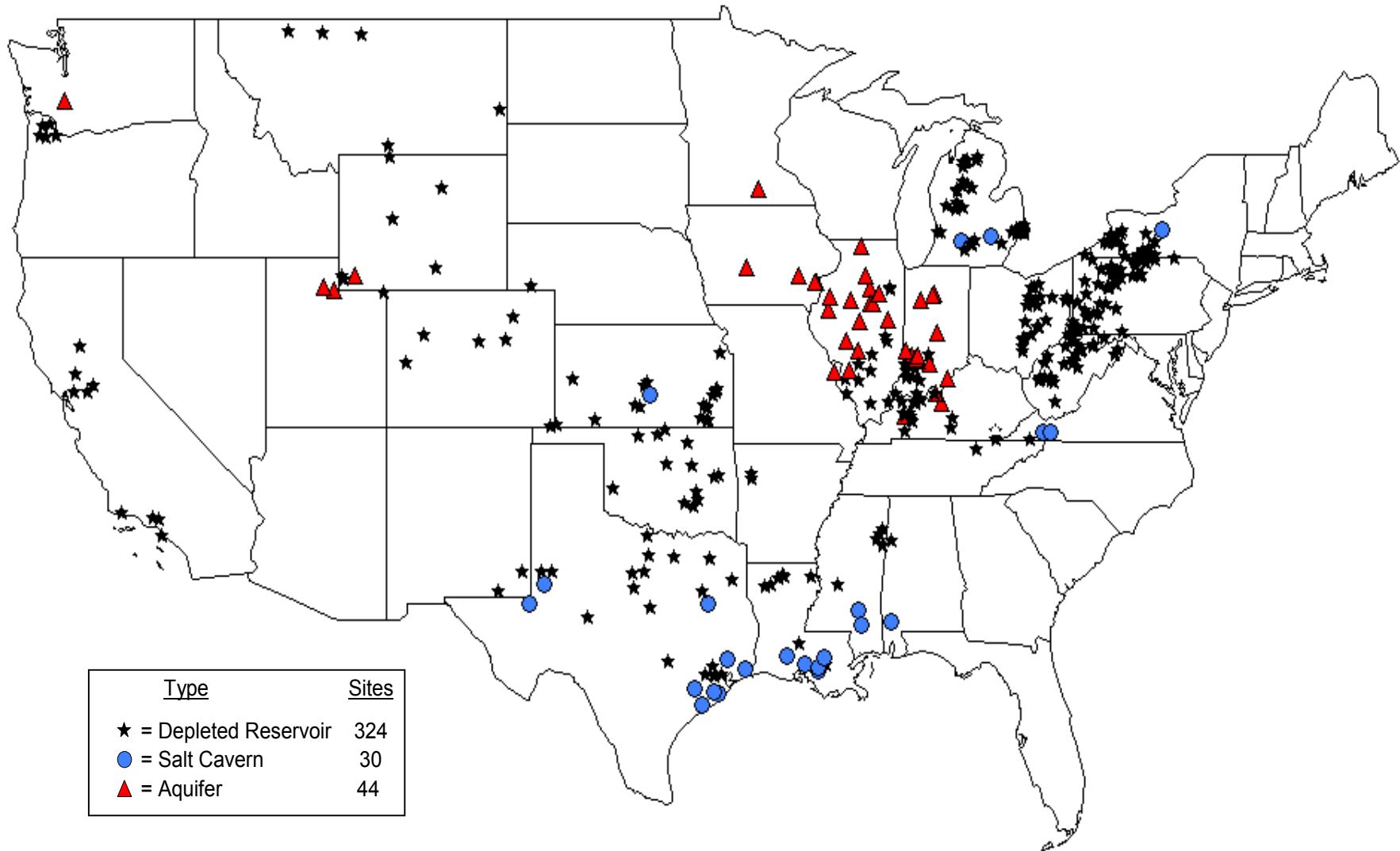
Figure 14. Locations of Existing Natural Gas Underground Storage Fields in the United States, 2007
