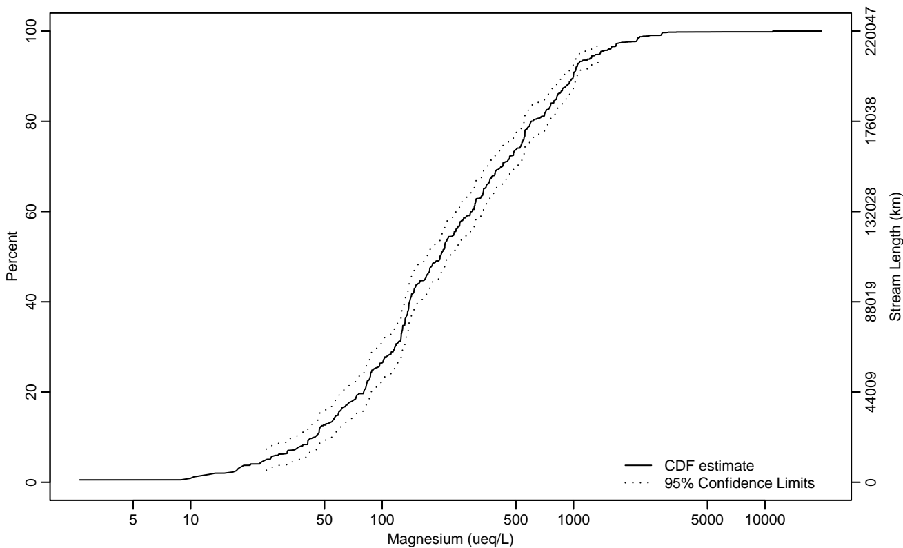
Summary Statistics
