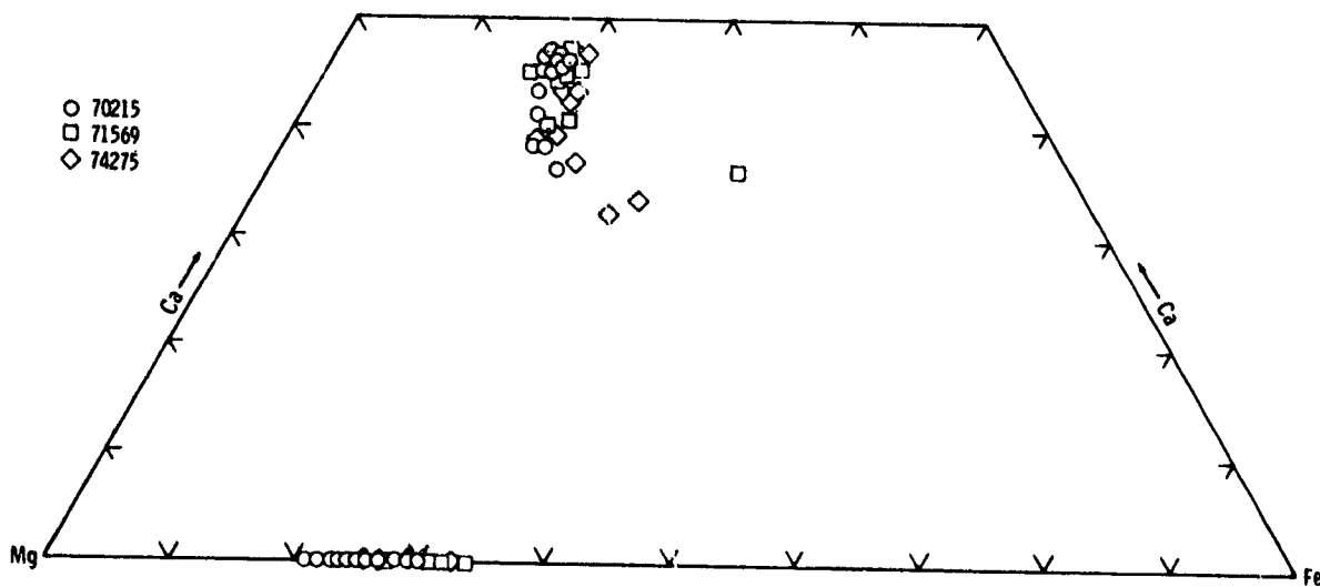
Figure 3-3.- Composition of olivine and pyroxenes in mare basalts 70215, 71569, and 74275.
