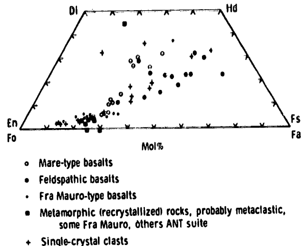
Figure 1-8.- 15015 pyroxenes and olivines from lithic and mineral clasts. (Di - diopside, Fs - ferrosilite, Fo - forsterite, En - enstatite, Fa - fayalite, Hd - hedenbergite.)
