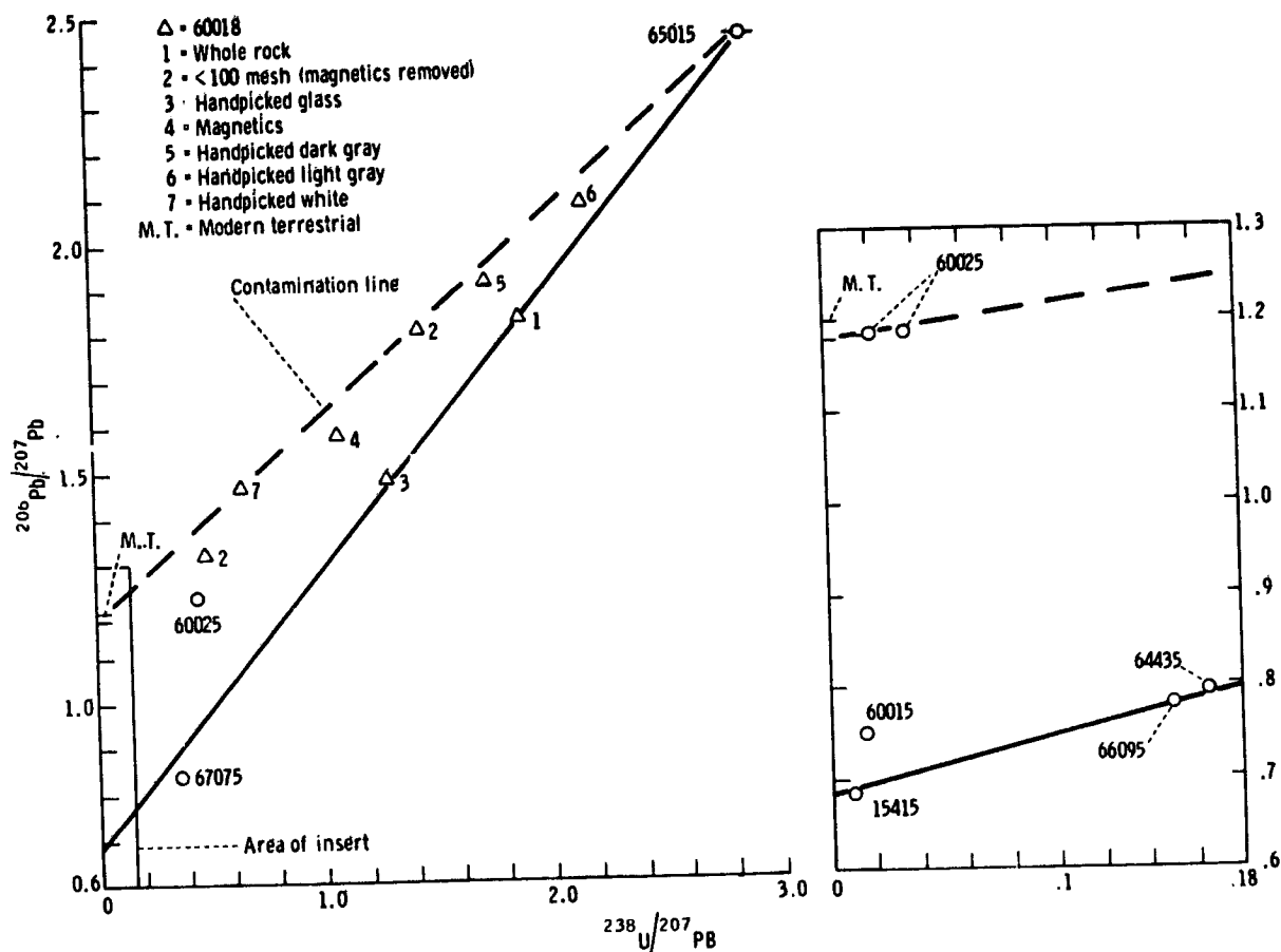
Figure 5-1.- A plot of ^{206}\text{Pb}/^{207}\text{Pb} compared to ^{238}\text{U}/^{207}\text{Pb} . New data from 60018, 60025, and 64435 are plotted. The following data are plotted for comparison: 60025 analyzed in reference 5-5, an interior analysis of anorthosite 60015 (ref. 5-1), breccia 66095 (ref. 5-2), anorthosite 15415 (refs. 5-6 and 5-7), anorthosite 67075 (ref. 5-8), and hornfels 65015 (ref. 5-1). Data are corrected for blanks only.
