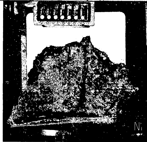
Figure 1-1.- Highly vesicular glassy breccia 15015.
