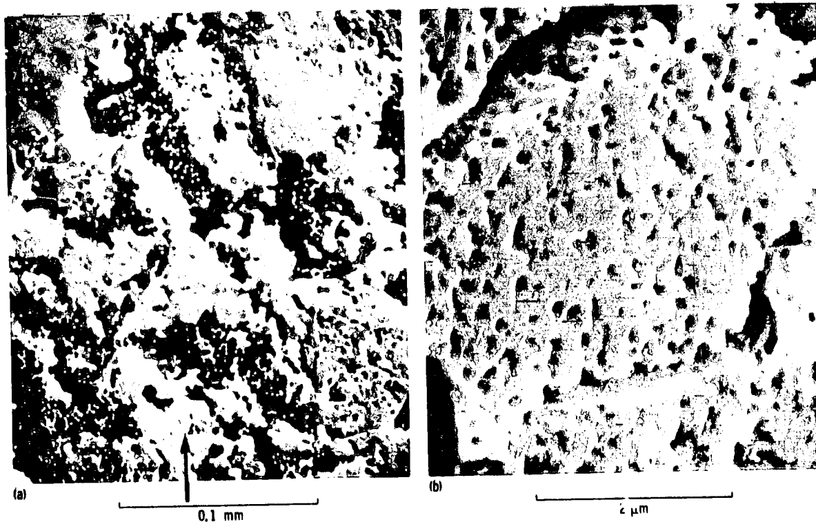
Figure 1-15. Scanning electron micrographs of a polished section that has been etched to reveal tracks in feldspars. (a) Aluminum X-ray scan superimposed on a backscattered electron scan. The arrow indicates the location of a feldspar grain of high track density in a rich Al-bearing mineral phase. (b) Micrograph of the same feldspar grain of high track density.
