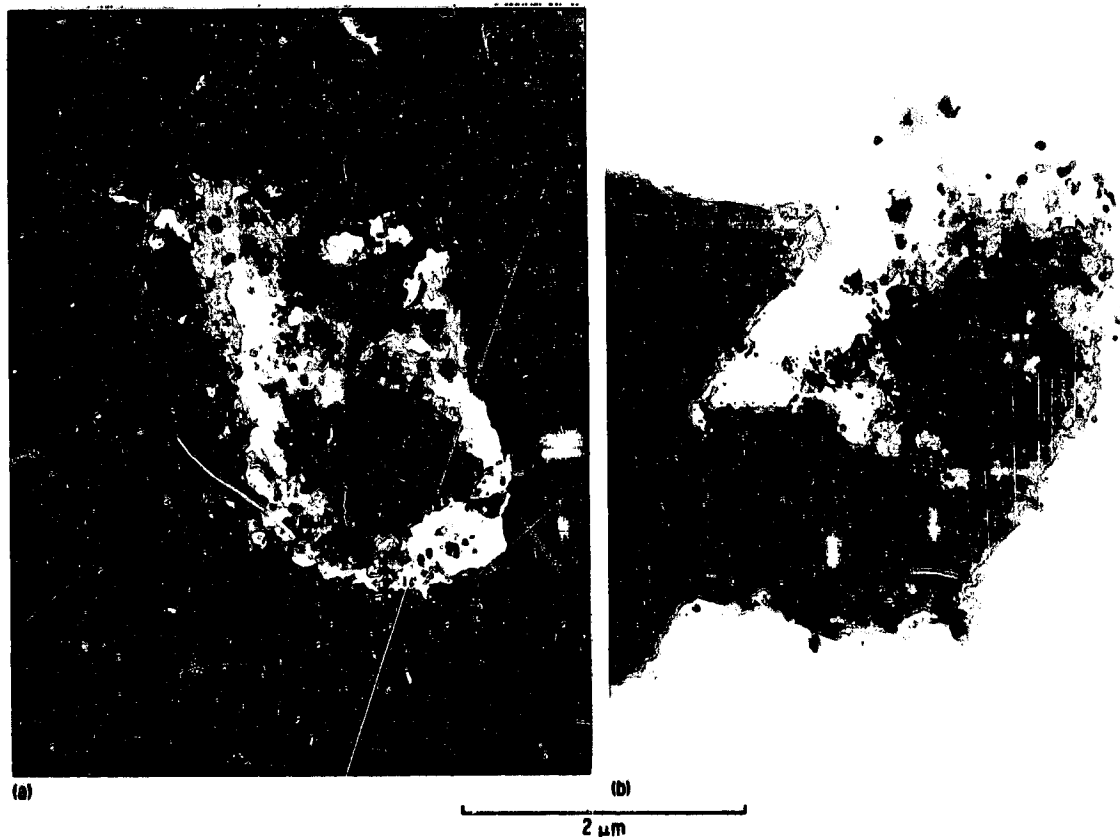
Figure 1-14.- 1-MeV electron micrographs of crystalline grains loaded with microcrystallites. (a) Dark field. (b) Bright field.
