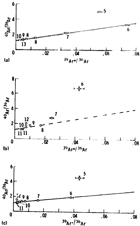
Figure 1-12.- Isochron diagram of ^{40}\text{Ar}/^{36}\text{Ar} and ^{39}\text{Ar}^{\#}/^{36}\text{Ar} for Ar from vesicular glasses 23c, 23d, and 26. The numbers represent temperature in units of 100^{\circ} C ( T_K = T_C + 273.15 ). The slopes of the isochron for 23c and 26 correspond to ages of 1.2 and 0.8 b.y., respectively. No correlation is observed for 23d, and the dashed line drawn corresponds to the same apparent age as 23c. The correlations appear to indicate outgassing of the glass or of inclusions within the glass within the last 1.0 b.y. It has been tentatively inferred that the glass formed at 1.0 b.y. or later, but the correlations could reflect recent solar heating. (a) Sample 15015.23c. (b) Sample 15015.23d. (c) Sample 25025.26.
