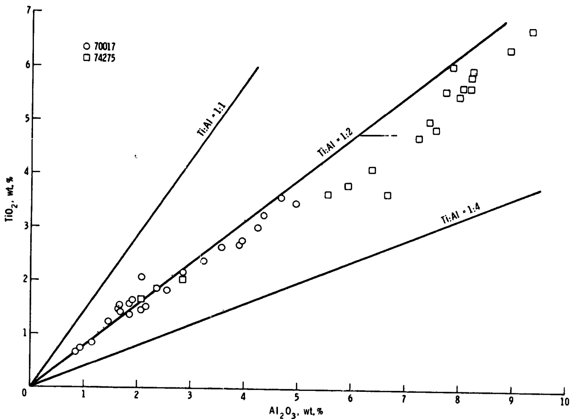
Figure 3-2.- \text{TiO}_2 and \text{Al}_2\text{O}_3 content of clinopyroxenes in mare basalts 70017 and 74275.
