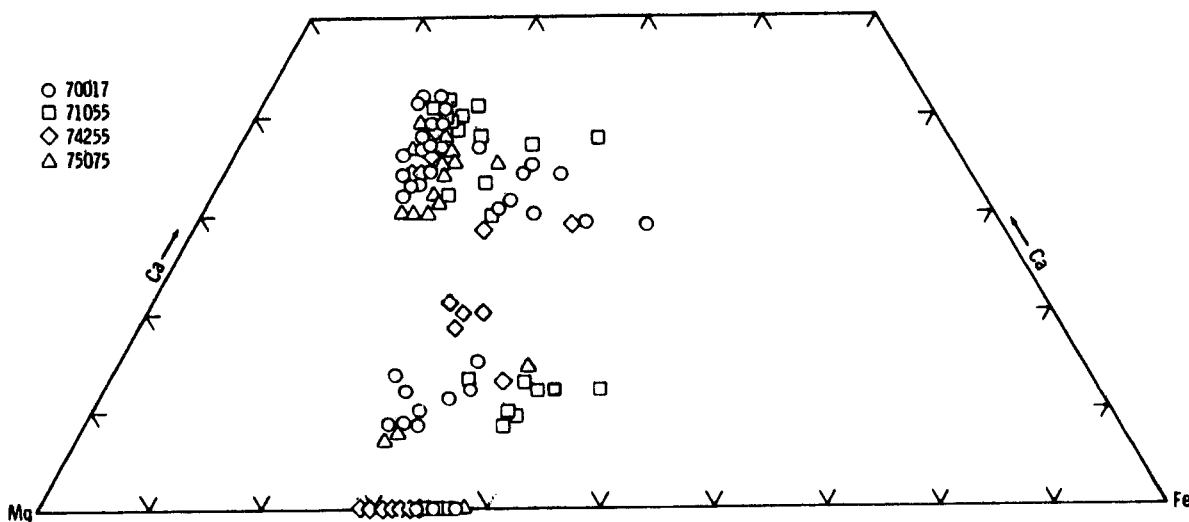
Figure 3-1.- Composition of olivine and pyroxenes in mare basalts 70017, 71055, and 75075.
