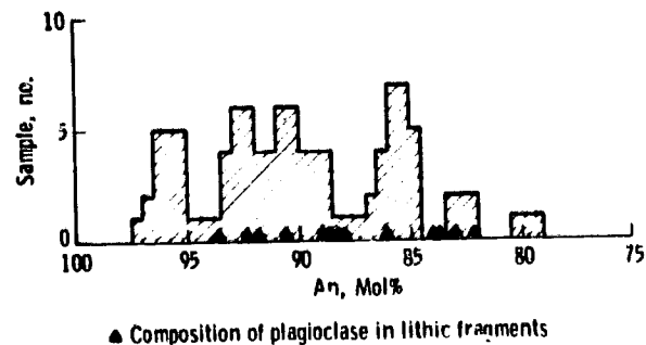
Figure 1-9.- 15015 histogram of plagioclase compositions in mineral clasts, size 100 to 400 \mu m.
