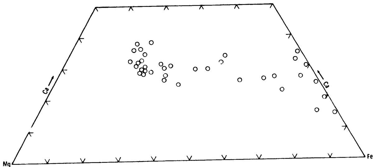
Figure 3-4.- Composition of pyroxenes and pyroxferroite in mare basalt 75035.
