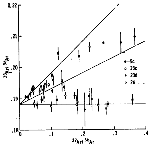
Figure 1-13.- Correlation diagram of ^{38}\text{Ar}/^{36}\text{Ar} and ^{37}\text{Ar}/^{36}\text{Ar} for matrix 5c and glasses 23c, 23d, and 26. The Ar is a mixture of trapped Ar ( ^{38}\text{Ar}/^{36}\text{Ar} = 0.188 , ^{37}\text{Ar}/^{36}\text{Ar} = 0 ) and cosmogenic Ar produced predominantly from the bombardment of Ca ( ^{38}\text{Ar}/^{36}\text{Ar} \approx 1.6 , ^{37}\text{Ar}/^{36}\text{Ar} \neq 0 , inversely proportional to exposure age). For all samples, the low-temperature release lies on a horizontal line, reflecting the absence in these (Ca) sites of cosmogenic ^{38}\text{Ar}_c and ^{36}\text{Ar} . The higher temperature points show the release of cosmogenic ^{38}\text{Ar}_c and ^{36}\text{Ar} in amounts approximately proportional to the amount of ^{37}\text{Ar} (= Ca). The upper line corresponds to an exposure age of 1000 m.y. irradiation coefficient ( J = 0.0298 ) or 1160 m.y. ( J = 0.0256 ). The slope of the middle line corresponds to an exposure age of half this. The absence of cosmogenic Ar in the low-temperature points appears to be at odds with the observations of radiogenic ^{40}\text{Ar} (fig. 1-12).
