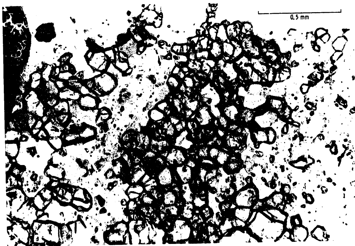
Figure 4-2.- Ordinary light photomicrograph of troctolite clast 8A showing polycrystalline aggregates of olivine and plagioclase.
