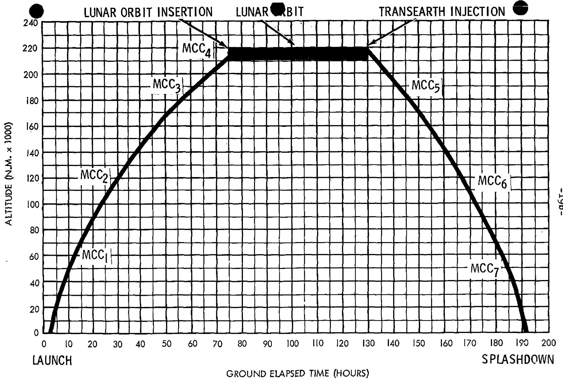
SPACECRAFT ALTITUDE VS. TIME
