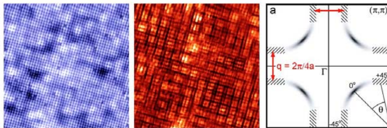
Figure 7 Left panel: 40nm square topographic image of Na-Ca 2 CuO 2 Cl 2 showing the square lattice of Cl atoms which are directly above the Cu sites. Center panel: Simultaneous 40nm-square LDOS image at -24meV: the LDOS patterns seen at three different dopings ( p = 0.08 ( T_c=0 ), 0.10 ( T_c=15 K), 0.12 ( T_c=21 K)) are almost identical. Right panel: ARPES reveals that the LDOS modulations are caused by scattering across the narrow neck of the Fermi surface with q=2\pi/4a_0 .
