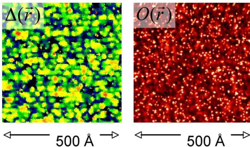
Left: The nanoscale superconducting energy gap disorder in \text{Bi}_2\text{Sr}_2\text{CaCu}_2\text{O}_x . Right: A simultaneous image of the dopant atom locations from SI-STM.
