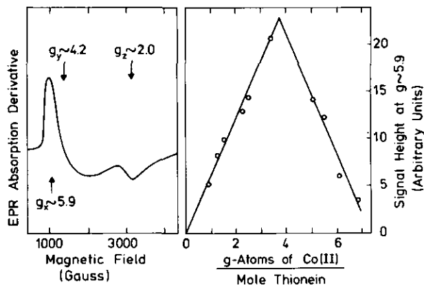
FIGURE 7. Electron spin resonance (ESR) titration of rabbit liver apometallothionein with \text{Co(II)} : (left) ESR spectrum of \text{Co(II)}_7 -metallothionein at 4°K, (right) dependency of ESR signal height at g_x \approx 5.9 on \text{Co(II)} -to-protein ratio (60).
