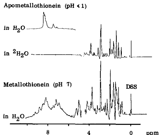
FIGURE 11. 270-MHz ^1\text{H-NMR} spectra of (bottom) equine metallothionein-1A and (top) apometallothionein. To obtain the spectra in \text{H}_2\text{O} , the solvent signal was suppressed by a gated pulse (75).
