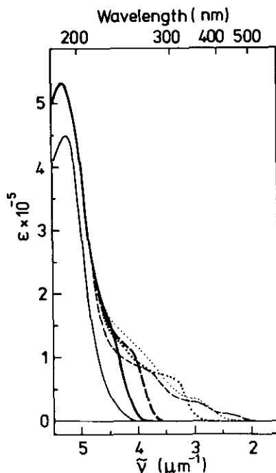
FIGURE 5. UV absorption spectra of (—) apometallothionein at pH 2, and of metallothionein at pH 8 containing a full complement (7 moles per mole) of (---) zinc, (- -) cadmium (· · ·) mercury, (- · -) bismuth and (- - -) lead (55).
