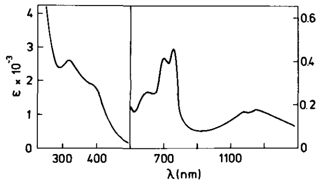
FIGURE 6. Absorption spectrum of rabbit liver \text{Co(II)}_7 -metallothionein in 0.05 M Tris-HCl, pH 7. The molar absorptancy refers to the metal (58).
