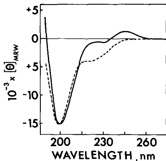
FIGURE 9. Circular dichroism spectra of (—) human liver \text{Zn(II)} -metallothionein (MT-2) in 0.05 M sodium phosphate buffer, pH 7.0; (---) human apometallothionein in 0.02 M perchloric acid, pH 1.7 Ordinate: mean residue ellipticity ( [\theta]_{\text{MRW}} ) refers to a mean residue weight of 99 (67).
