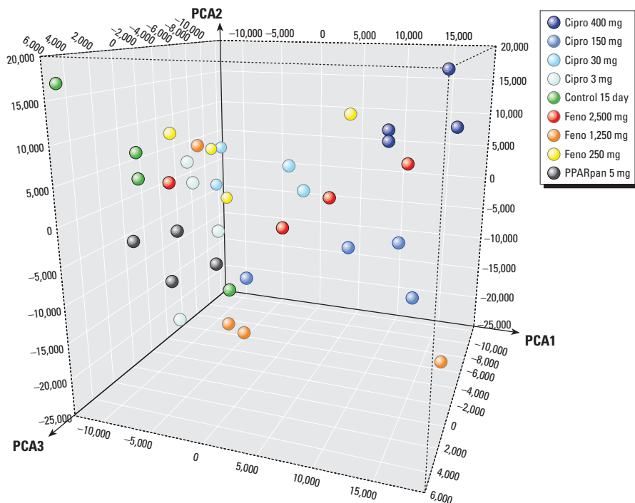
Figure 1. PCA of gene expression signals (expressed as arbitrary units) in cynomolgus monkey liver samples after 15-day treatment with hyperlipidemia drugs. Cipro, ciprofibrate; Feno, fenofibrate.
