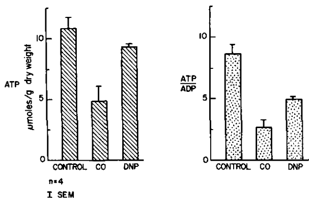
FIGURE 2. ATP content and ATP/ADP in isolated perfused rat lungs under control conditions and during ventilation with 95% CO 2 (CO) or perfusion with 0.8mM dinitrophenol (DNP). At the end of 60-90 min of perfusion, lungs were rapidly frozen at the temperature of liquid N 2 , extracted with cold ethanolic perchloric acid, and assayed for adenine nucleotide content by enzyme methods (5).
