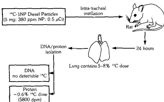
FIGURE 4. Disposition of ^{14}\text{C} from 1-nitro[ ^{14}\text{C} ]pyrene vapor-coated onto diesel particles. Rats were treated with ^{14}\text{C} -1NP vapor-coated onto diesel particles by intratracheal instillation with the particles. Animals were maintained for 24 hr after dosing, then the lungs were removed and analyzed for total ^{14}\text{C} content. DNA and protein were isolated and ^{14}\text{C} bound to these macromolecules was measured as described in "Materials and Methods."
