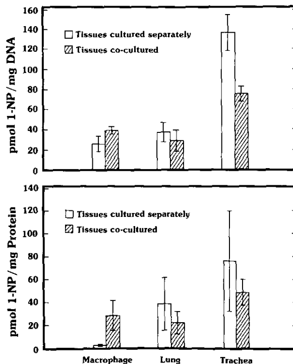
FIGURE 2. Binding of 1-nitro ^{14}\text{C} pyrene metabolites to DNA and protein. Cultures of rabbit alveolar macrophages ( 0.5 \times 10^6 cells/mL), lung tissue 31.0 mg/mL, or tracheal tissue (14.0 mg/mL) were incubated 20 hr in tissue culture media containing ^{14}\text{C} -1NP (8.1 \mu\text{M} ; 81.0 nCi/mL). Cellular DNA (A) and protein (B) were isolated for analysis of binding as previously described. Similarly, rabbit alveolar macrophages ( 0.5 \times 10^6 cells/mL), lung tissue 29.0 mg/mL and tracheal tissue (14.0 mg/mL) were co-cultured 20 hr in media containing ^{14}\text{C} -1NP (8.1 \mu\text{M} ; 81.0 nCi/mL). The cells and tissues were separated from one another as described and prepared for analysis of DNA and protein binding. Data are presented as the mean of three experiments \pm standard error of the mean.
