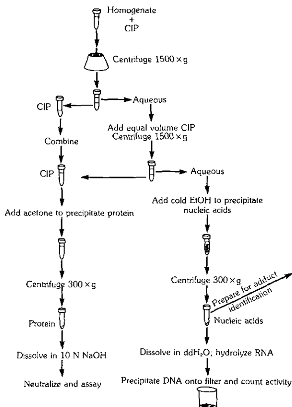
FIGURE 1. DNA isolation scheme. Protein was removed from cellular nucleic acid by two extractions of the cell lysates or tissue homogenates with chloroform:isoamyl alcohol:phenol (CIP, 24:1:25). Protein in the CIP portion was precipitated with acetone and DNA in the aqueous portion was precipitated with cold ethanol. After residual protein and RNA were hydrolyzed with proteinase K and NaOH, respectively, DNA was acid precipitated onto glass fiber filters and associated radioactivity measured in a liquid scintillation spectrometer. Samples used for identification of DNA adducts were not taken through the hydrolysis procedure, but were prepared directly as described in "Materials and Methods."
