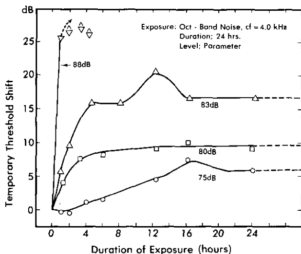
FIGURE 1. Temporary threshold shifts (TTS) as a function of the duration of exposure produced by an octave-band SPL of the noise centered at 4.0 kHz. The parameter is the octave-band SPL of the noise. Measurements of TTS were made about 4 min ( TTS_4 ) after a subjects had been recovered from the noise. For the 88 dB exposure, some subjects had TTS's greater than 25 dB after 1-2 hr of the exposure. Therefore, the exposure was terminated (7).
