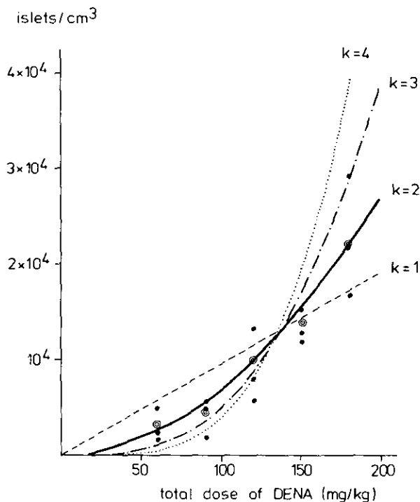
FIGURE 5. Multi-hit model for the induction of ATP-ase deficient cell clones in rat liver by carcinogens (43). The model equation is:
