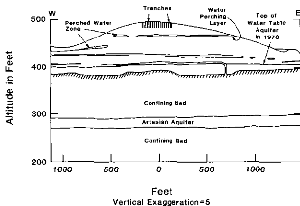
FIGURE 1. Conceptual diagram of contaminant percolation below the disposal trenches.
