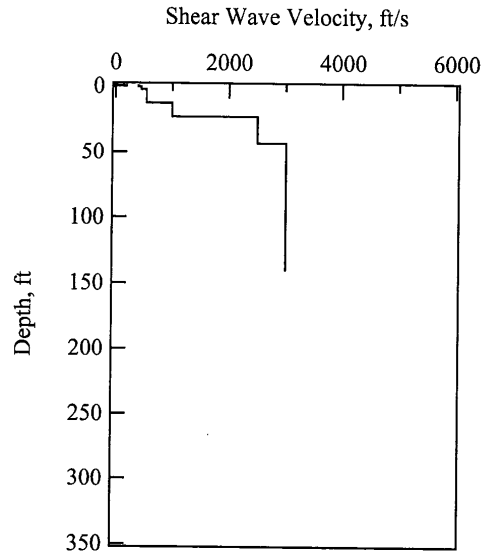
c. SASW-29 Shear Wave Velocity Profile
