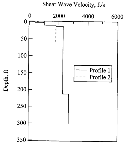
c. SASW-34+36 Shear Wave Velocity Profile
