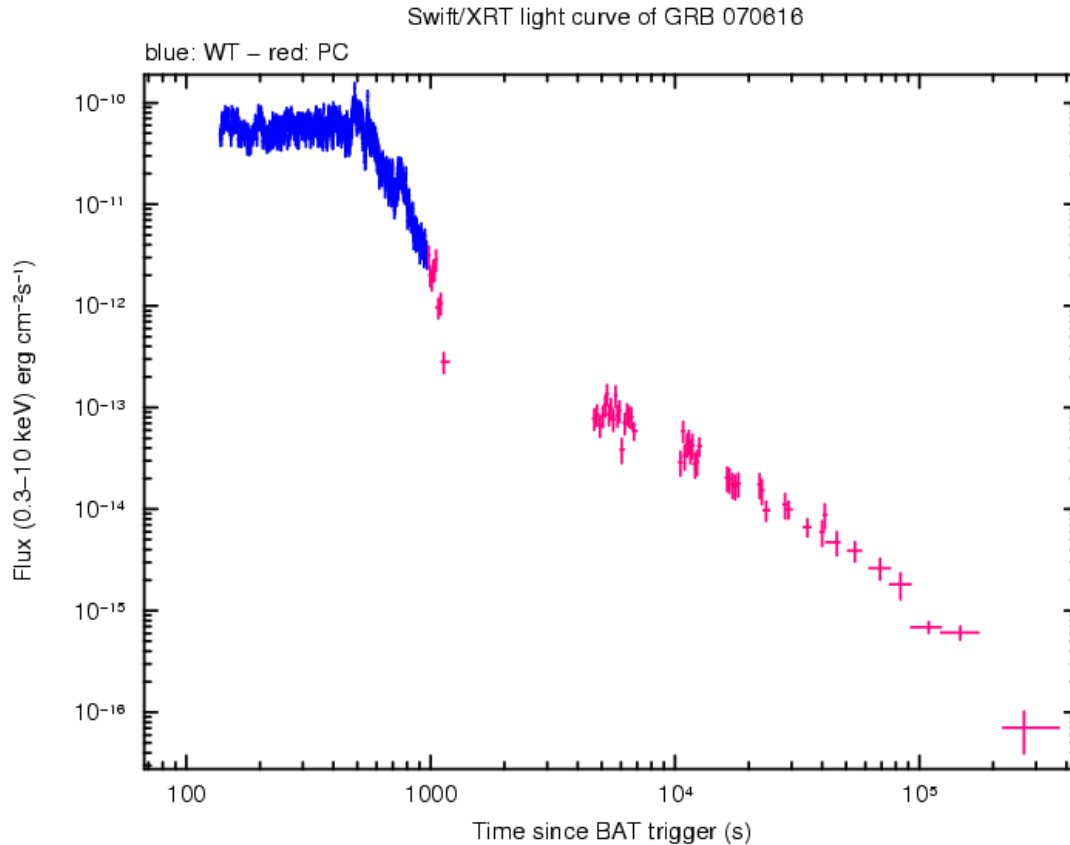
Figure 2: XRT fluxed lightcurve in the 0.3-10 keV band. Power law fits are described in the text. The approximate count rate to flux conversion is 1 \text{ count s}^{-1} = 4.5 \times 10^{-13} \text{ erg cm}^{-2} \text{ s}^{-1} , based on the spectrum from orbit 2 onwards.
