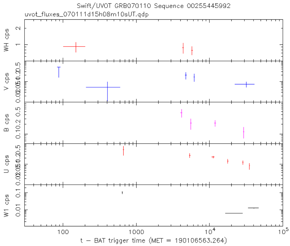
Figure 4: UVOT light curve in five filters. Here "WH" is a white filter and "W1" is UVW1.
