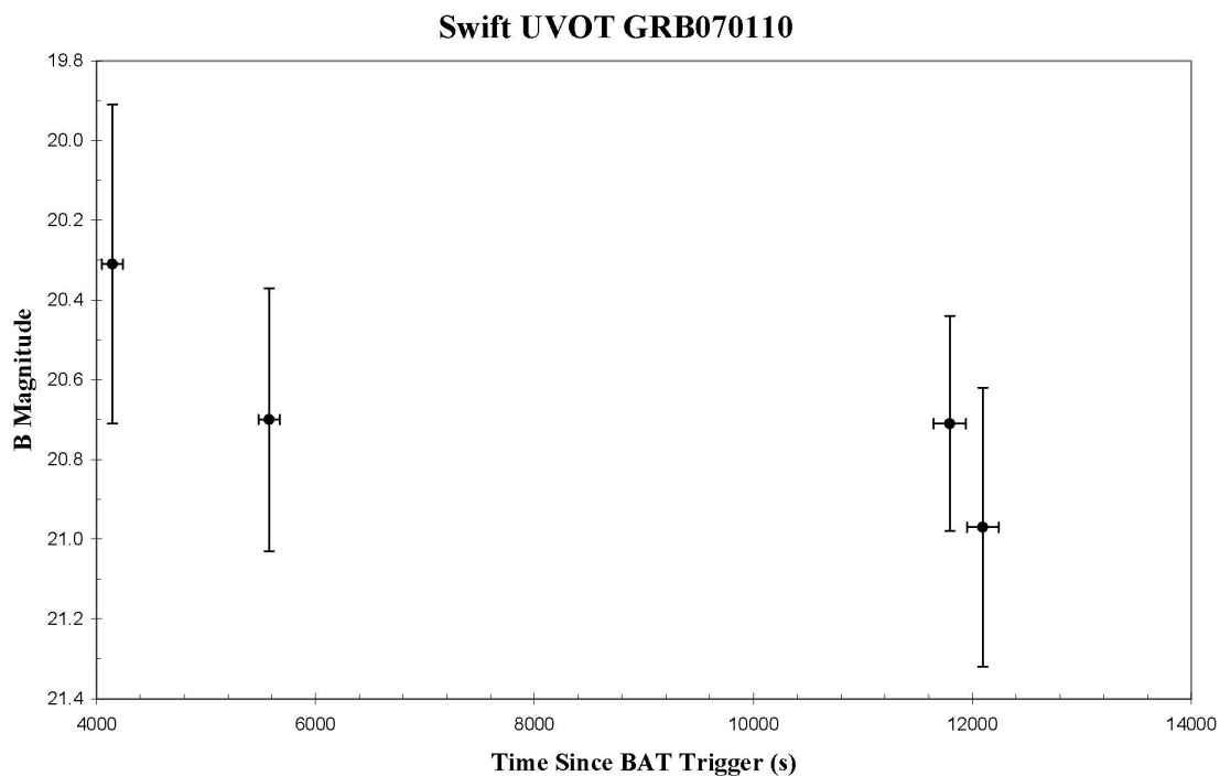
Figure 4: UVOT B-band light curve.
