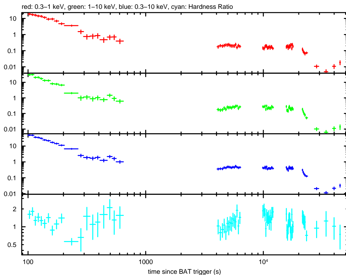
Figure 3: XRT Hardness Ratio and Light curve in three energy bands. The hardness ratio is the counts ratio: C(1-10 \text{ keV})/C(0.3-1 \text{ keV}) and the time scale is the same as in Figure 2.
