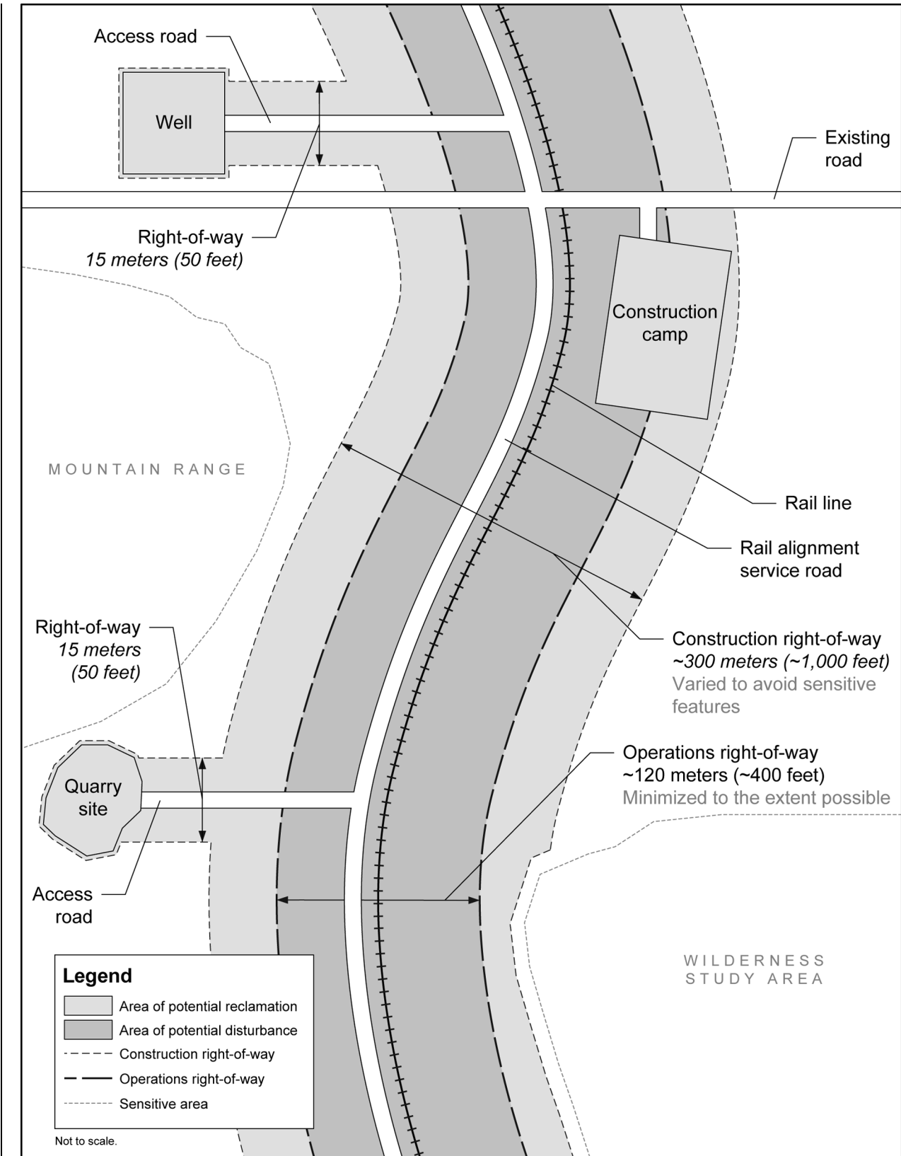
Figure 2-3. The construction and operations rights-of-way.
