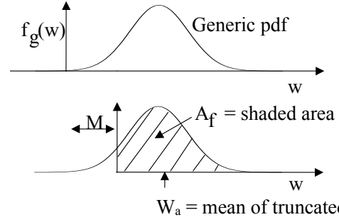
Figure 2. Schematic of generic distribution of snow water equivalent showing effect of uniform melt depth M on the distribution.
