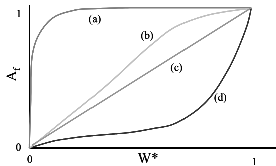
Figure 3. Depletion curves derived for four distributions: (a) normal, CV=0.1, (b) lognormal, CV=0.75, (c) exponential, (d) gamma, skew=4.7.
