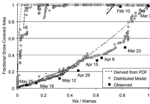
Figure 4. Depletion curve for Upper Sheep Creek derived by three methods, (1) From PDF of snow water equivalent on March 3, 1993, (2) from distributed model outputs, and (3) from observations. Note hysteresis in relationship as snow covers entire area with only slight accumulation in early season (on left and top), while melt uncovers areas gradually.
