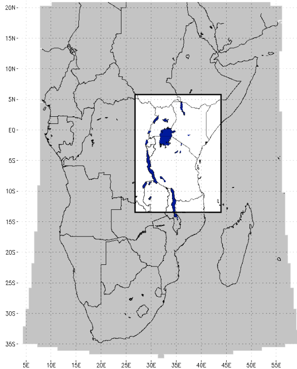
Figure 2. Map of the outer domain (gray) and inner domain (white) used in RAMS simulations for the CLIP project.
