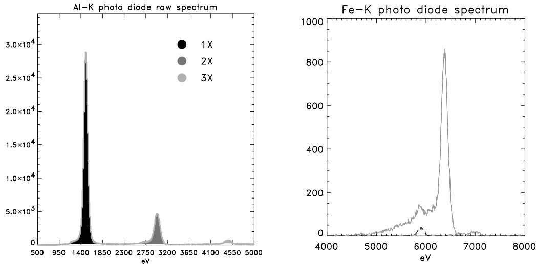
Figure 3. The left panel illustrates how we counted the X-ray events in a generic piled up spectrum: we weighted the events of the second and third piled up peaks by a factor of two and three respectively. In the right panel we plot a PD mode Fe-K spectrum (the grey line) which includes the contamination due to the corner source fluxes. A corner source spectrum (black dashed line) as observed in PC mode is also shown. The exposure is \sim 84 seconds with a count rate of \sim 250 counts \text{sec}^{-1} and in this case we estimate that the contamination from the corner source is \sim 3\% .
