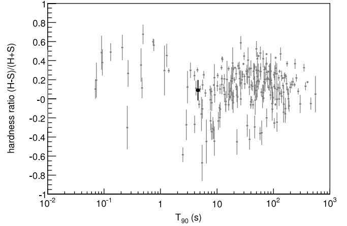
FIG. 2.—Plot of duration ( T_{90} ) and hardness ratio (HR) of 226 Swift bursts from GRB 041217 to GRB 070616. We define hardness ratio as (H - S)/(H + S) , where S and H are energy fluences in 15–50 and 50–150 keV, respectively. The values of T_{90} and hardness ratio for GRB 070610 ( large filled black circle ) are 4.6 \pm 0.4 s and 0.09 \pm 0.11 (90% confidence level), respectively.
