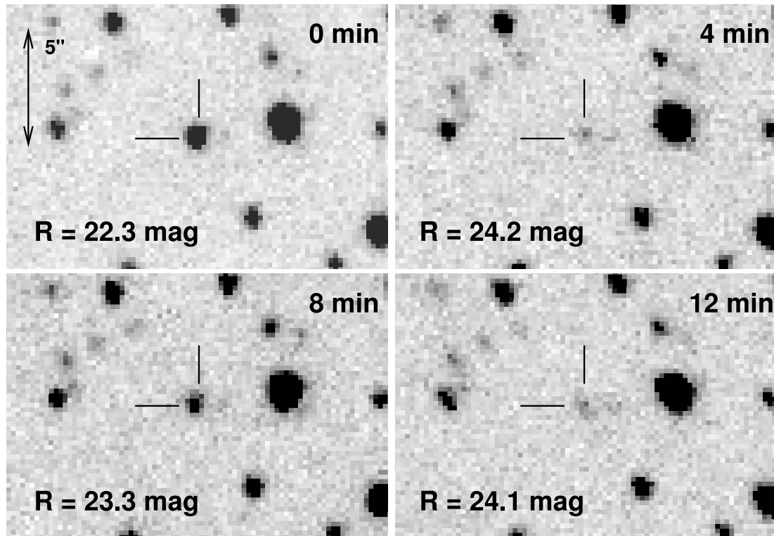
FIG. 8.—Close-up view of the optical field of the Swift J195509.6+261406 optical transient using the LRIS instrument on the Keck I 10 m telescope; 2007 June 15 starting at 12 : 33 UT. All four images were taken in the R -band with a 180 s exposure in sequence. The transient brightens by over 2 mag in only 3 minutes about 5 days after the burst trigger. Such rapid variability at late times is unprecedented from an extragalactic GRB optical afterglow.
