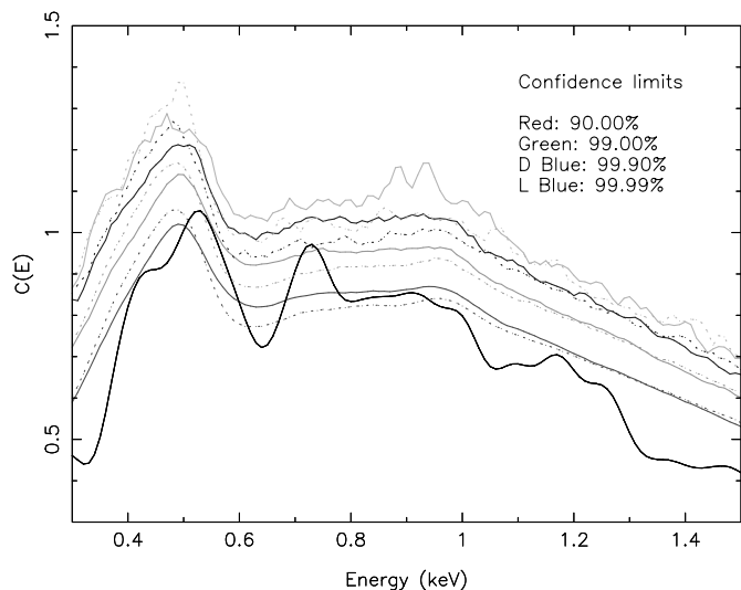
FIG. 8.—GRB 050730 ( T + 692 s to T + 792 s): RS comparison between the absorbed power law models containing a single N_{\text{H}} component (wabs, dotted lines) and two components (wabs and zwabs, solid lines). Note that the feature becomes far less significant with the addition of the N_{\text{H}} column at the appropriate redshift. [See the electronic edition of the Journal for a color version of this figure.]
