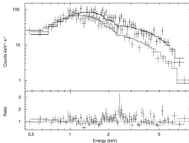
FIG. 24.—Spectra modeled with an absorbed power law model: GRB 060124 and GRB 060210 ( T + 119 s to T + 129 s). Note the residuals around 2.3 keV. [See the electronic edition of the Journal for a color version of this figure.]
