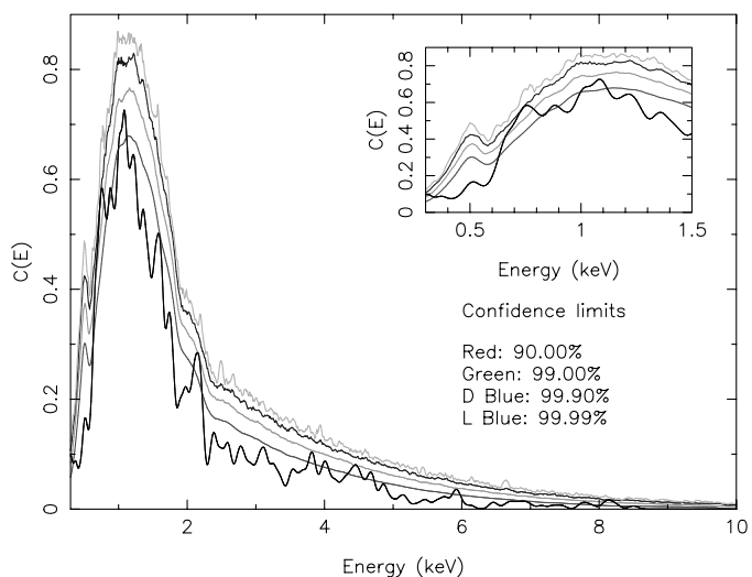
FIG. 9.—GRB 060109: RS results. [See the electronic edition of the Journal for a color version of this figure.]
