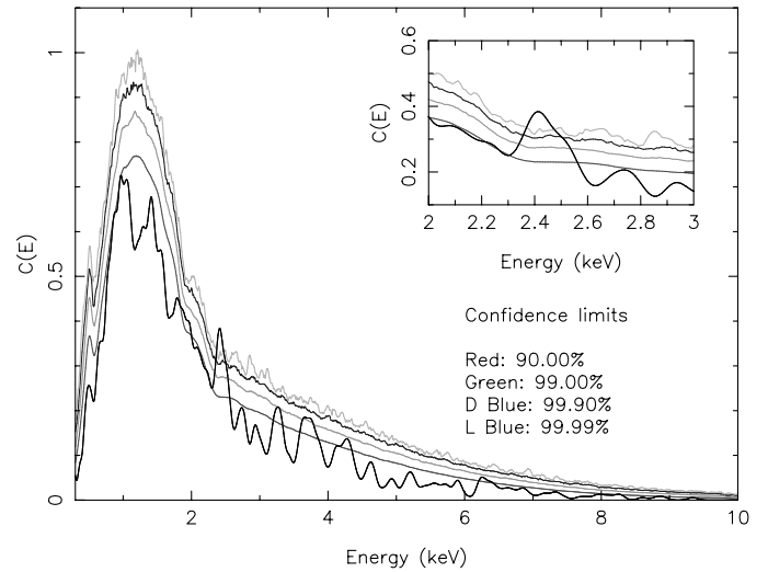
FIG. 18.—GRB 060418 ( T + 119 s to T + 129 s): RS results. [See the electronic edition of the Journal for a color version of this figure.]
