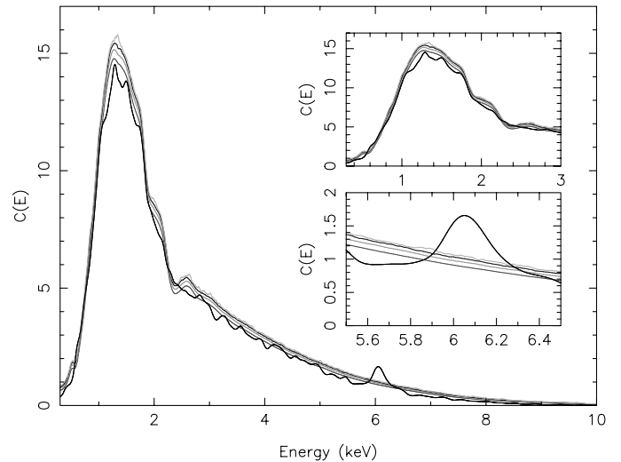
FIG. 3.—PKS 0745-19: RS method. Confidence contours mark the significance of the spectral features. Inset focus on energy ranges of interest. [See the electronic edition of the Journal for a color version of this figure.]
