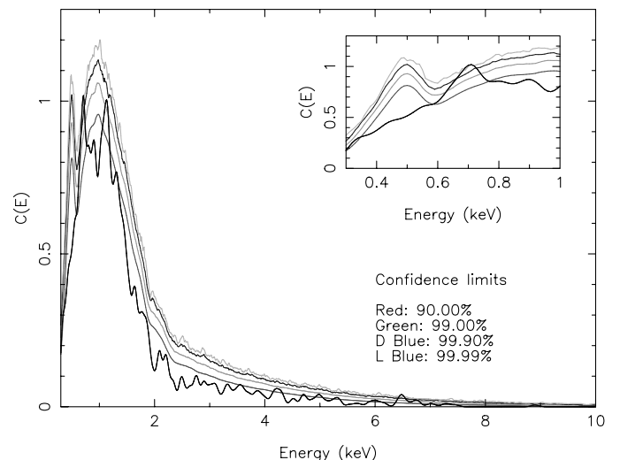
FIG. 19.—GRB 060418 ( T + 169 s to T + 194 s): RS results. [See the electronic edition of the Journal for a color version of this figure.]
