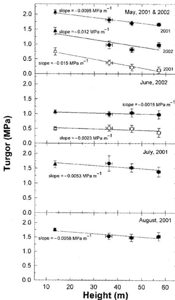
Figure 4. Pre-dawn (filled symbols) and midday (open symbols) turgor as a function of height on young (triangles) and old (circles) trees during the 2001 and 2002 growing seasons. Midday values were not available for sampling sessions when midday water potentials were not able to be collected. Bars represent standard errors for measurements on one sample from each of five trees ( n = 5 ).
