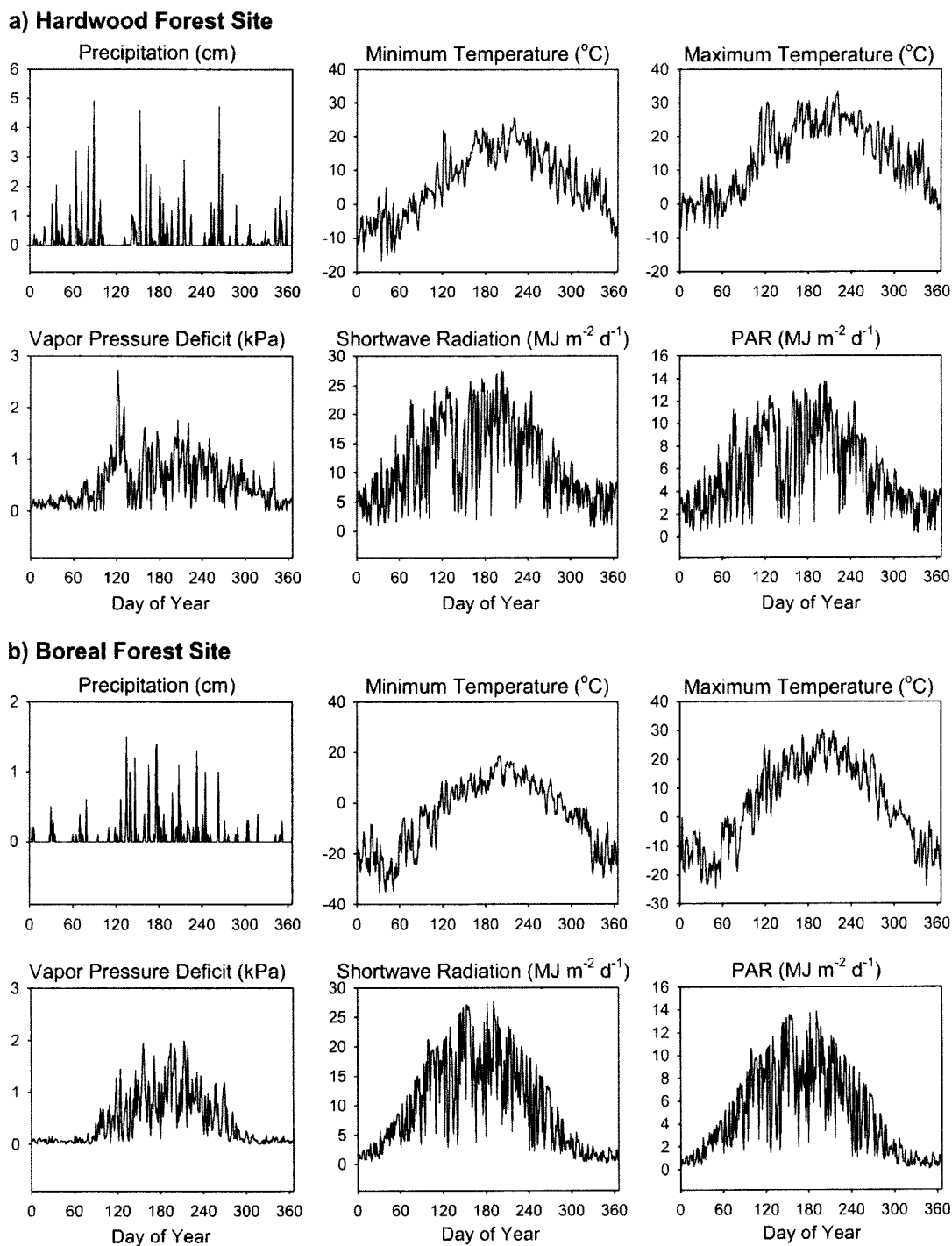
Fig. 2. Meteorological data used in model simulations: (a) Hardwood Forest site, (b) Boreal Forest site.
