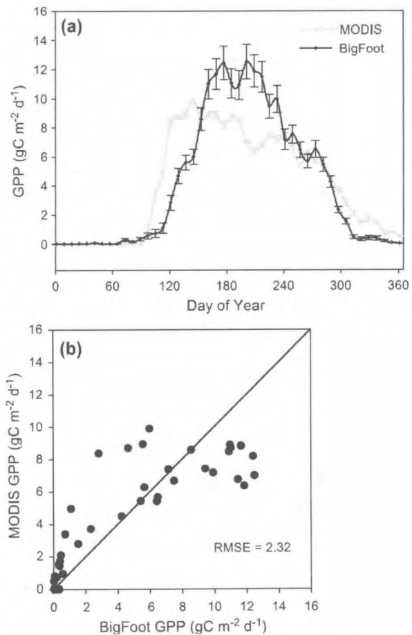
Fig. 5. Gross primary production estimates from MODIS and BigFoot at the Hardwoods site. Values are means and standard deviations for the twenty-five 1 km 2 cells in the BigFoot study area.
