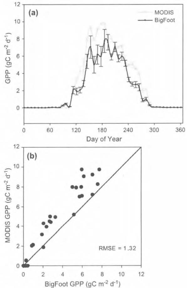
Fig. 11. Gross primary production estimates from MODIS and BigFoot at the Boreal Forest site. Values are means and standard deviations for the twenty-five 1\text{ km}^2 cells in the BigFoot study area.
