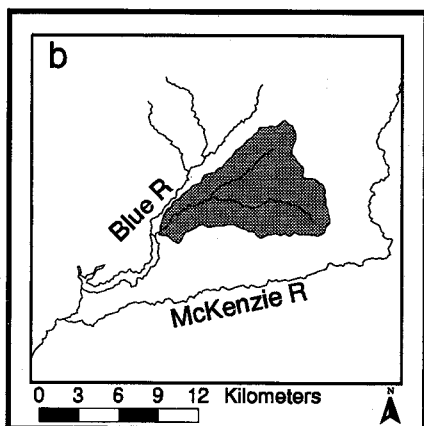
Figure 2. The Willamette River watershed in Oregon. (a) Map of Oregon showing the Willamette River. (b) Area of enlargement showing the west-flowing McKenzie River, a tributary to the Willamette River, and the Andrews Experimental Forest (shaded), which drains into the Blue River.
