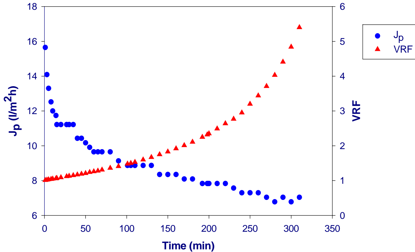
UF of kiwifruit juice. Time course of permeate flux and VRF (batch concentration mode; T = 25\text{ }^\circ\text{C} ; TMP = 0.85\text{ bar} ; Q_f = 800\text{ l/h} )
