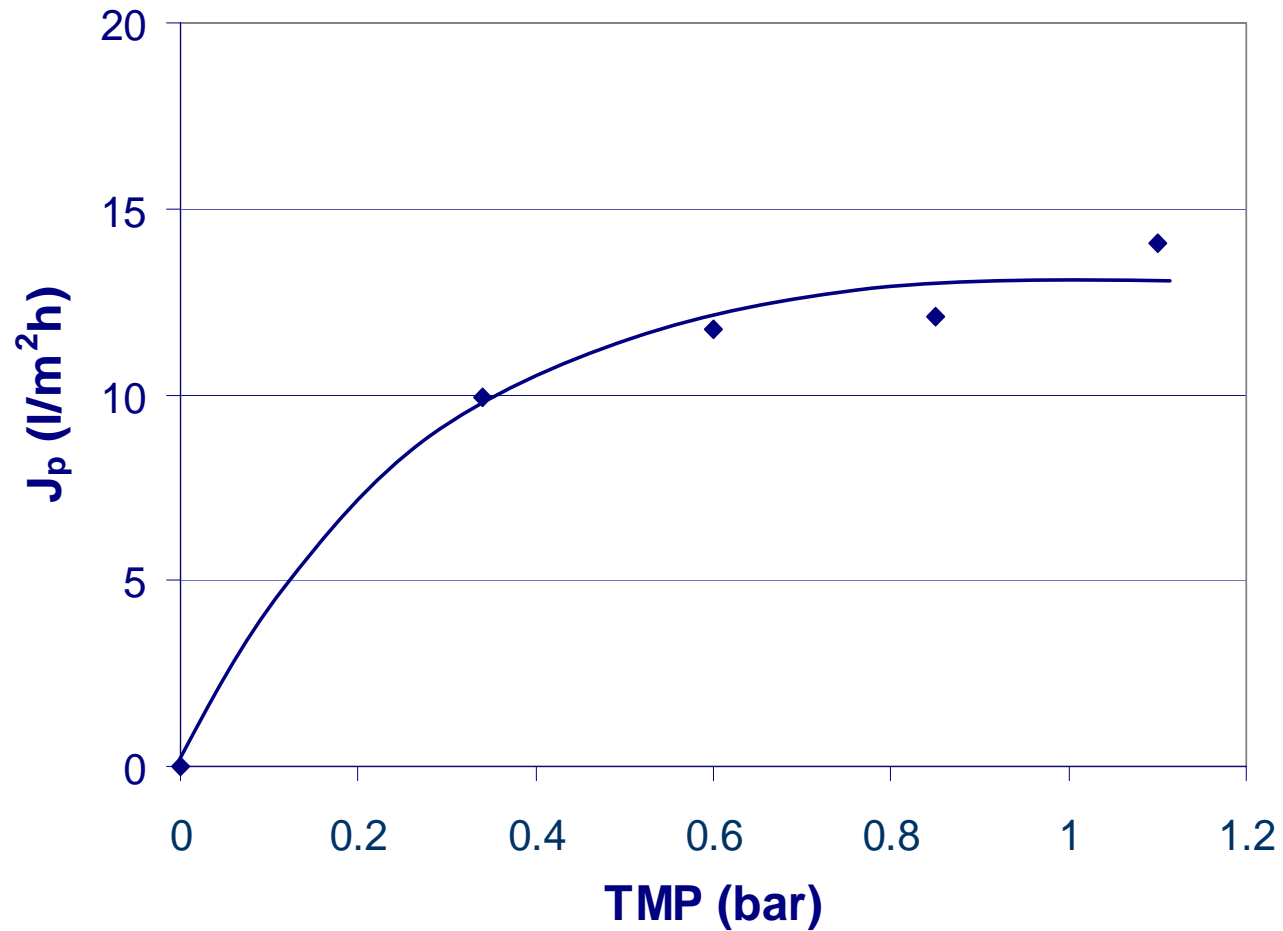
UF of kiwifruit juice. Permeate flux vs. TMP
