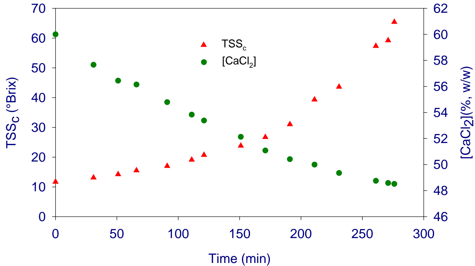
OD of clarified kiwifruit juice. Time course of TSS and brine concentration
