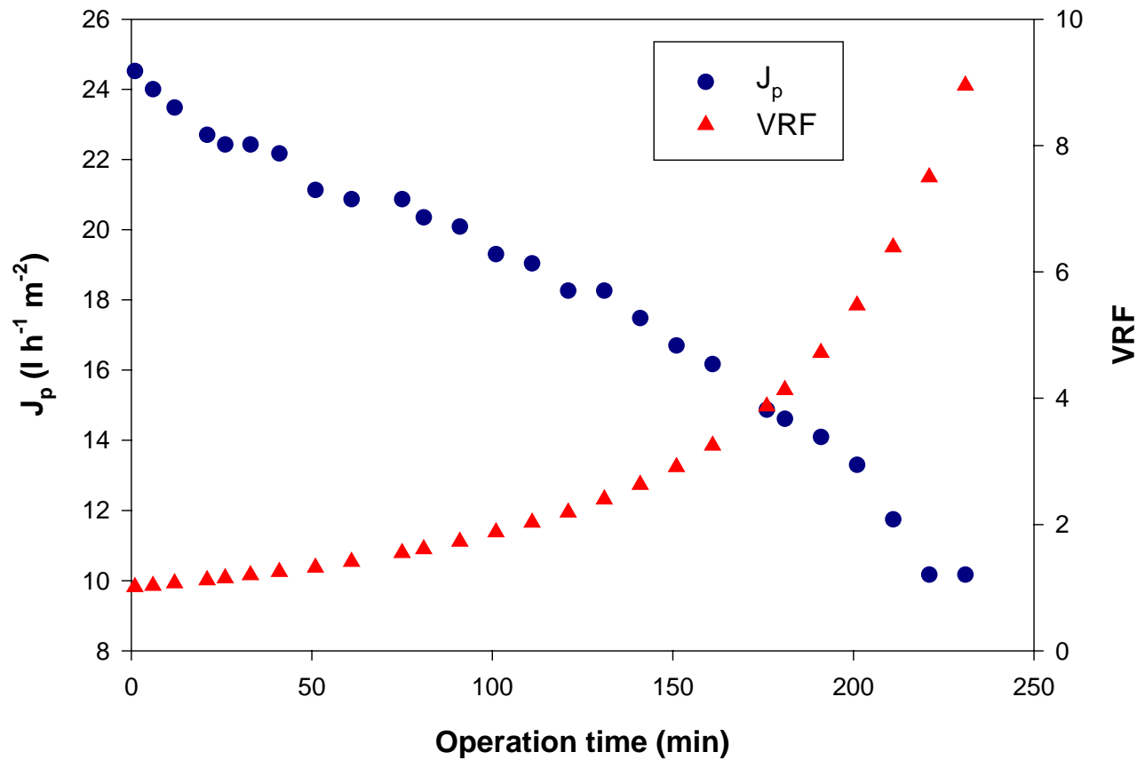
UF of carrot juice. Time course of permeate flux and VRF (Operating conditions: T = 23.5\ ^\circ\text{C} ; Q_f = 800\ \text{l/h} ; \text{TMP} = 1.03\ \text{bar} )
