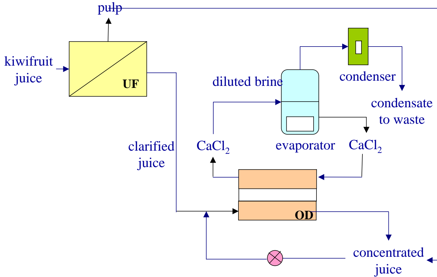
Integrated membrane process for the production of concentrated kiwifruit juice
