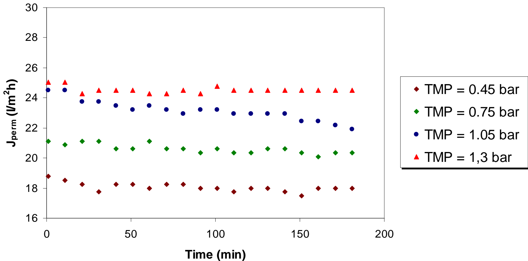
Ultrafiltration of carrot juice Time course of permeate flux at different operating TMPs Operating conditions: T = 23.5 \text{ }^\circ\text{C} ; Q_f = 800 \text{ l/h}
