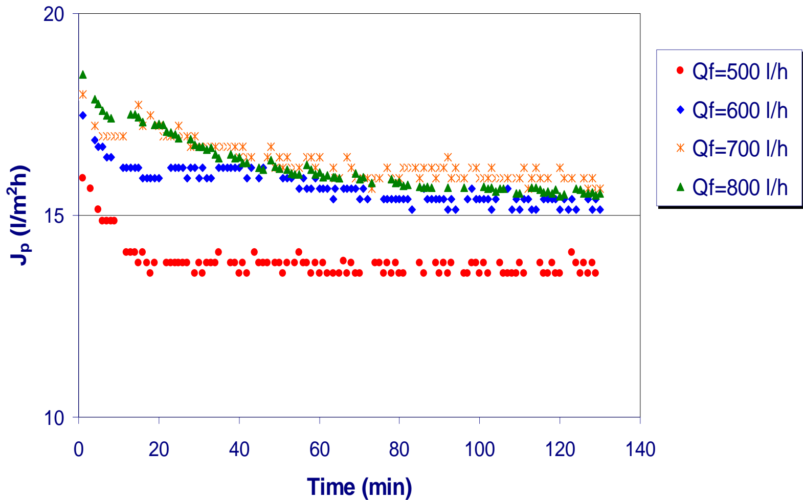
Time course of permeate flux at different axial feed flow rates ( TMP = 0.85 \text{ bar} ; T = 25 \text{ }^\circ\text{C} )
