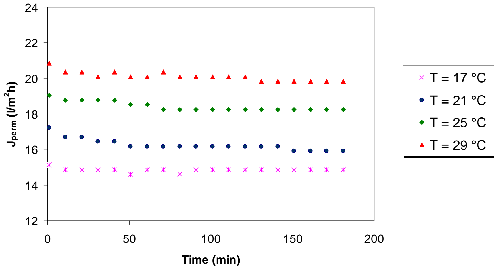
Ultrafiltration of carrot juice Time course of permeate flux at different temperatures Operating conditions: TMP = 0.85 bar; Q f = 800 l/h
