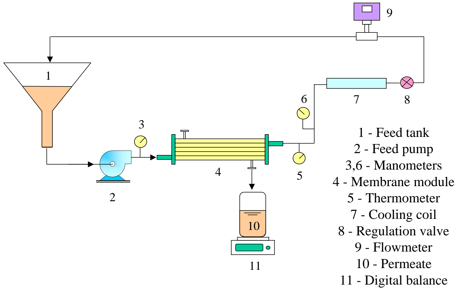
UF laboratory pilot plant
