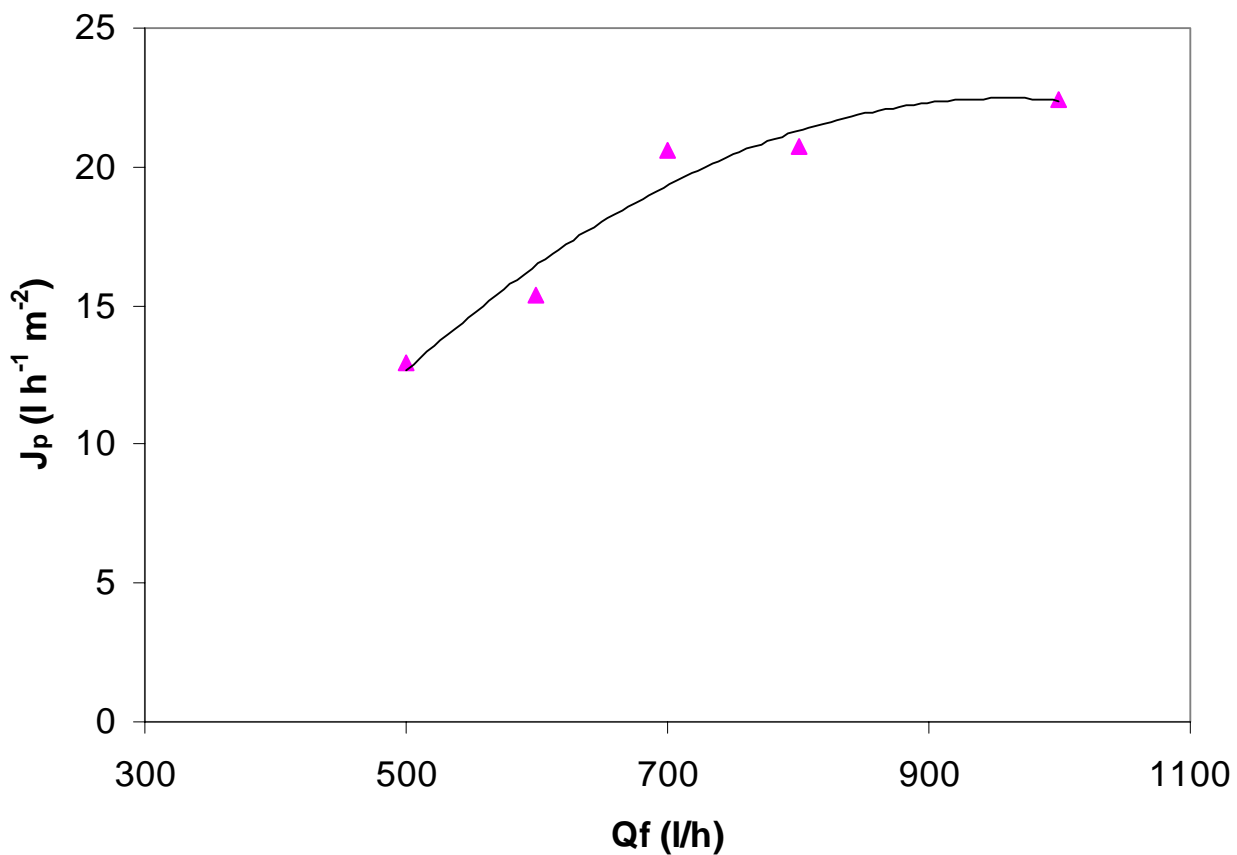
UF of carrot juice. Effect of the axial flow rate on the permeate flux (Operating conditions: T = 23.5 °C; TMP = 0.85 bar)
