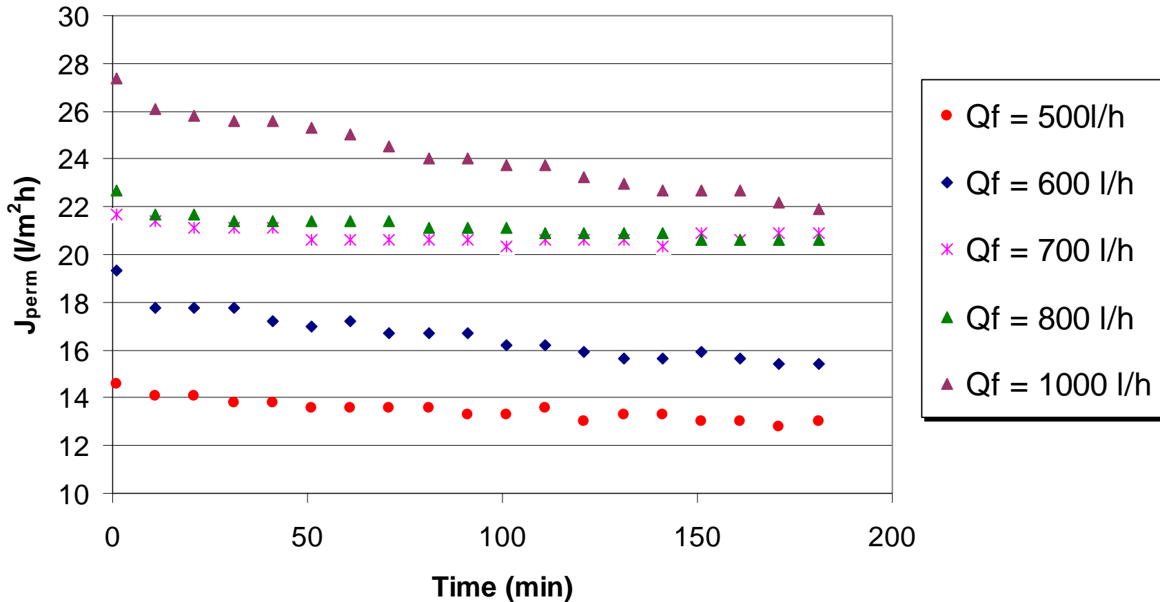
Ultrafiltration of carrot juice Time course of permeate flux at different axial flow rates Operating conditions: T = 23.5 °C; TMP = 0.85 bar
