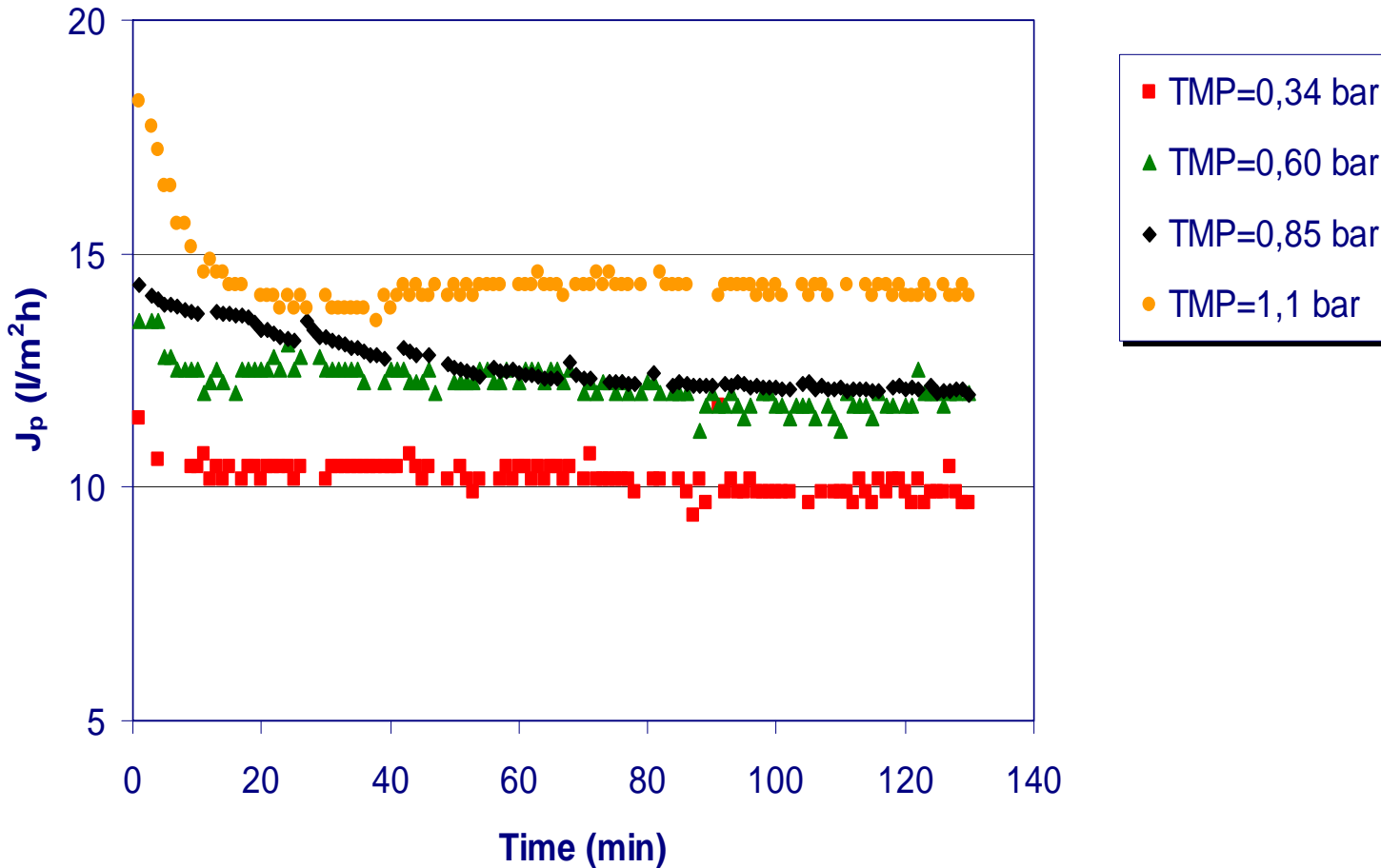
UF of kiwifruit juice. Time course of permeate flux at different TMP ( T = 25\text{ }^\circ\text{C} ; Q_f = 800\text{ l/h} )
