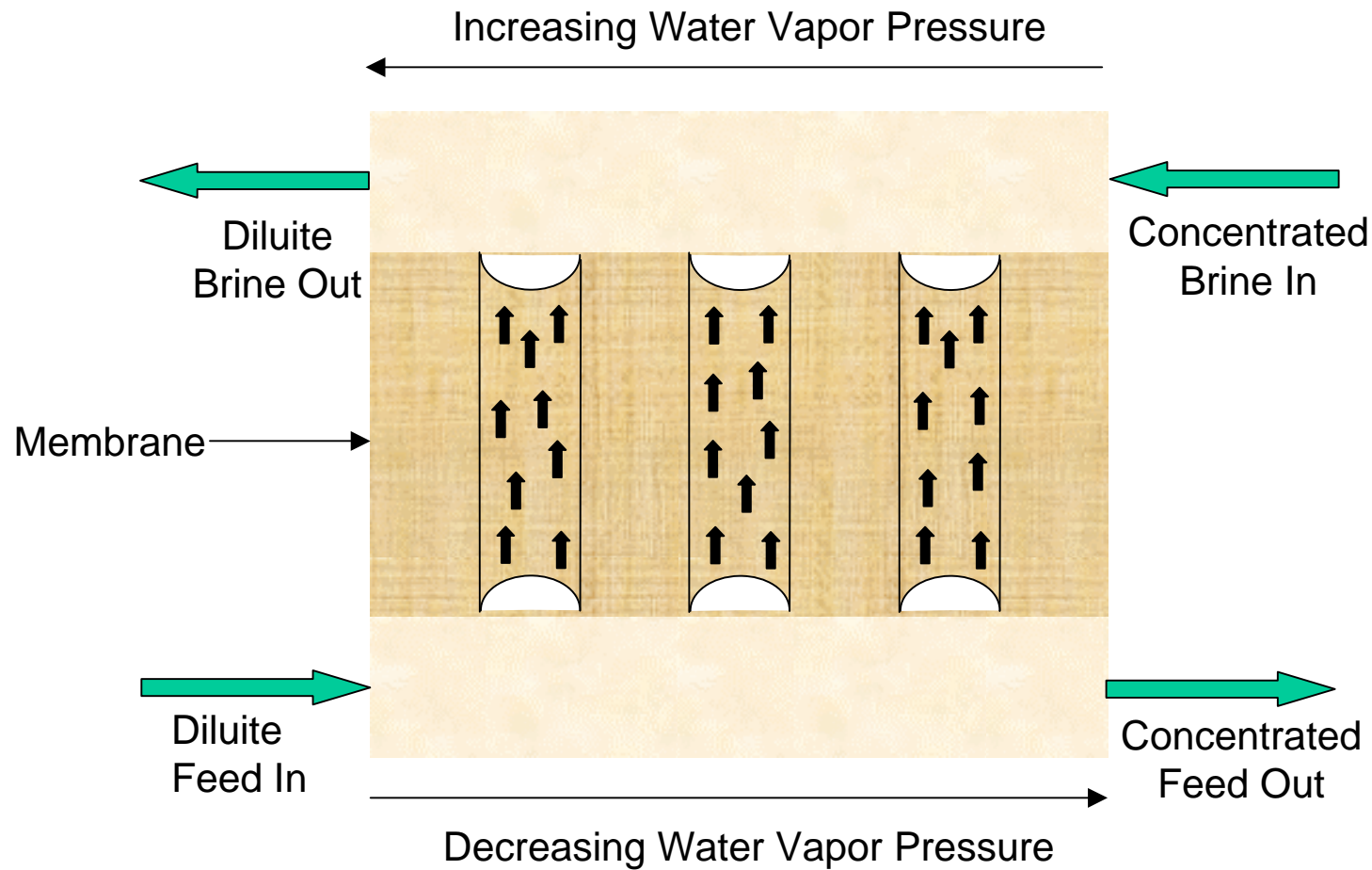
Mechanism of osmotic distillation through a microporous hydrophobic membrane (Hogan et al., 1998)
