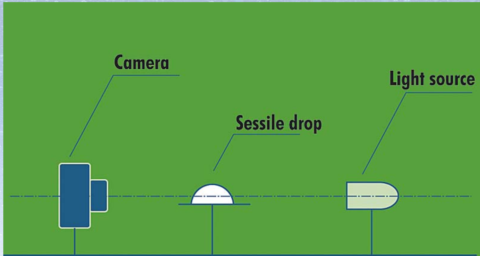
Principle of contact angle determination
