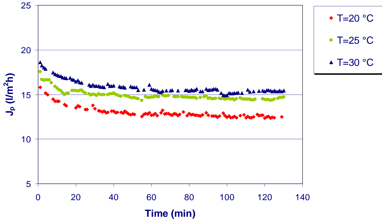
UF of kiwifruit juice. Time course of permeate flux at different temperatures ( TMP = 0.85\text{ bar} ; Q_f = 800\text{ l/h} )
