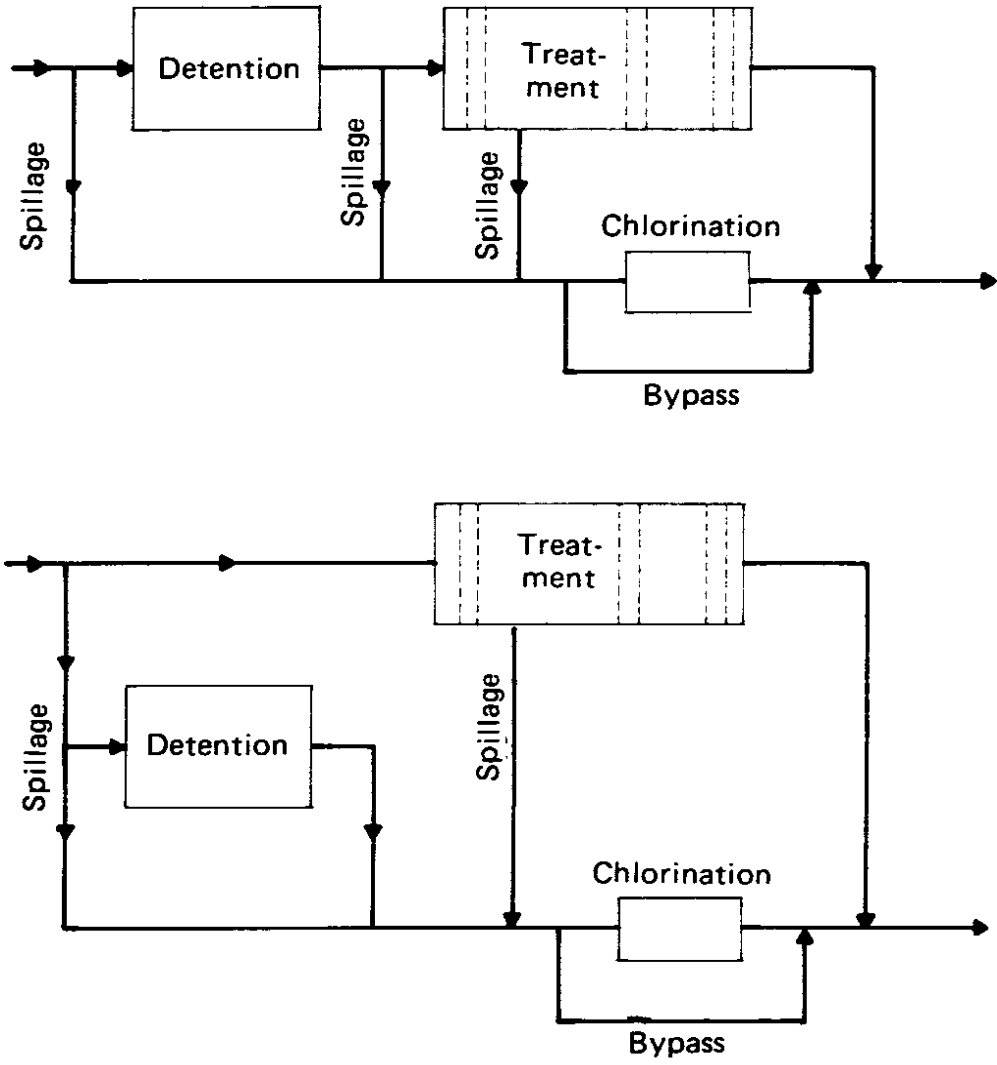
Figure A-3 Treatment processes simulated by Storage Treatment Block of SWMM
