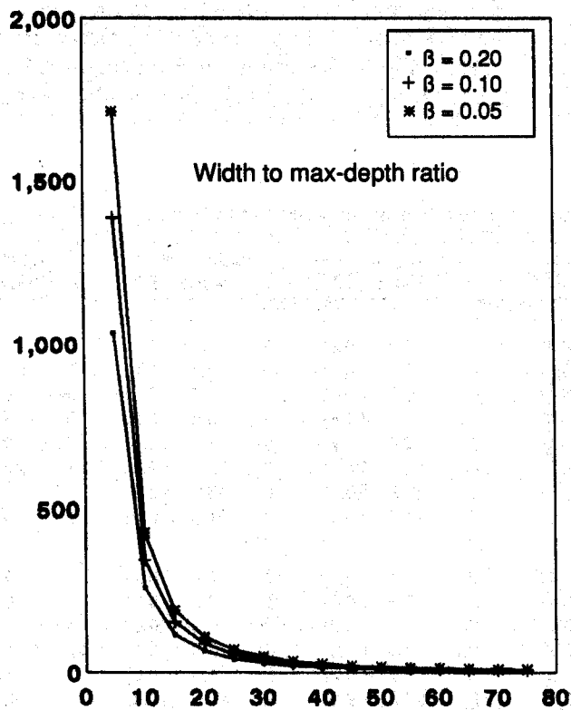
Figure 3—Sample sizes required to detect differences for various levels of \beta in all habitat types combined.
