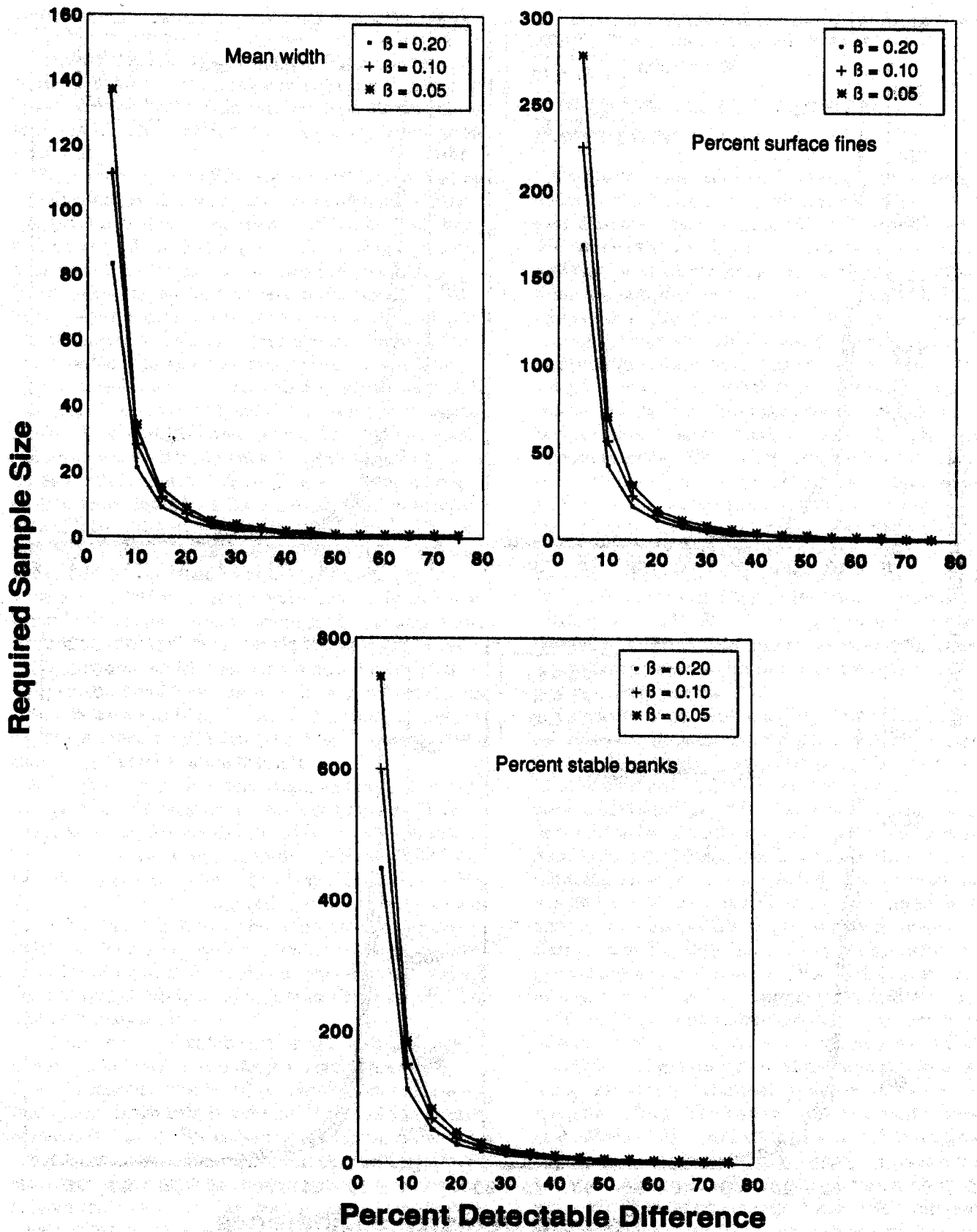
Figure 4—Sample sizes required to detect differences for various levels of \beta in riffle habitats only.
