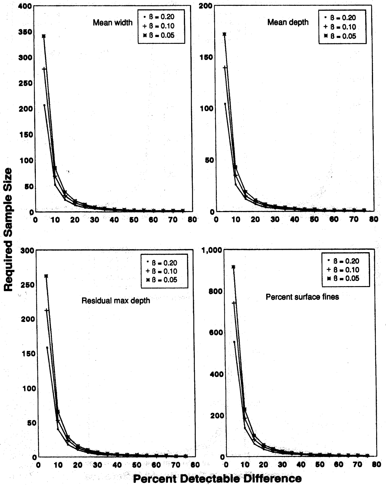
Figure 5—Sample sizes required to detect differences for various levels of \beta in pool habitat types only.
