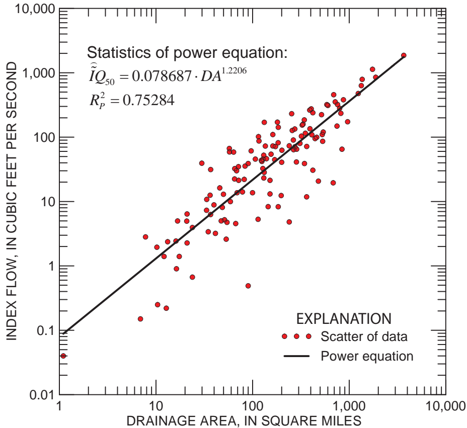
Figure 4. Relation between estimates of index flow from gaging station records, \hat{I}Q_{50} , and drainage area ( DA ) [ R_p^2 , the Pearson coefficient of determination].
