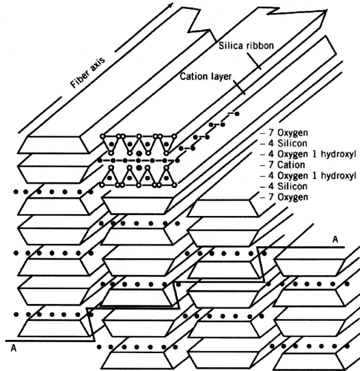
Figure 5. Microscopic structure of amphibole fibers (22). Reprinted with permission.
