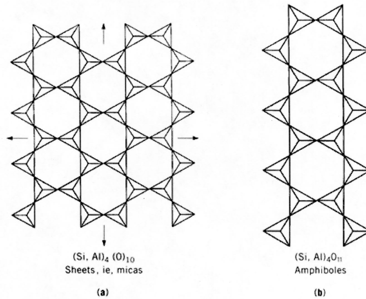
Figure 3. Silicate backbones of chrysotile and amphiboles: (a) the sheet silicate structure of chrysotile, analogous to that of micas; (b) the double-chain silicate structure found in amphiboles (4). Courtesy of Oxford University Press.
