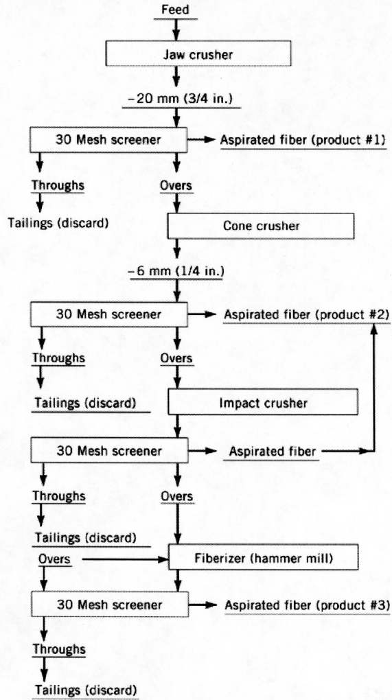
Figure 9. Schematic of a typical asbestos milling flowline (30 mesh = 590 \mu\text{m} ) (35).
