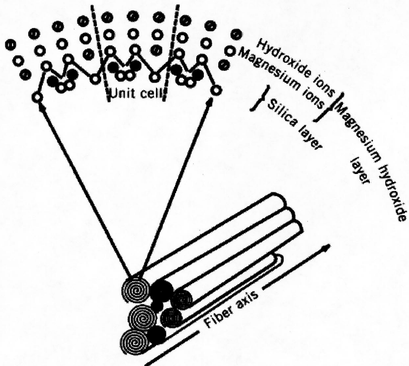
Figure 4. Microscopic structure of chrysotile fibers (3). Reprinted with permission.
