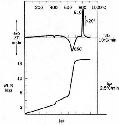
Figure 7. Thermal analysis curves for asbestos: (a) chrysotile; (b) crocidolite (in inert atmosphere) (3). Reprinted with permission.
