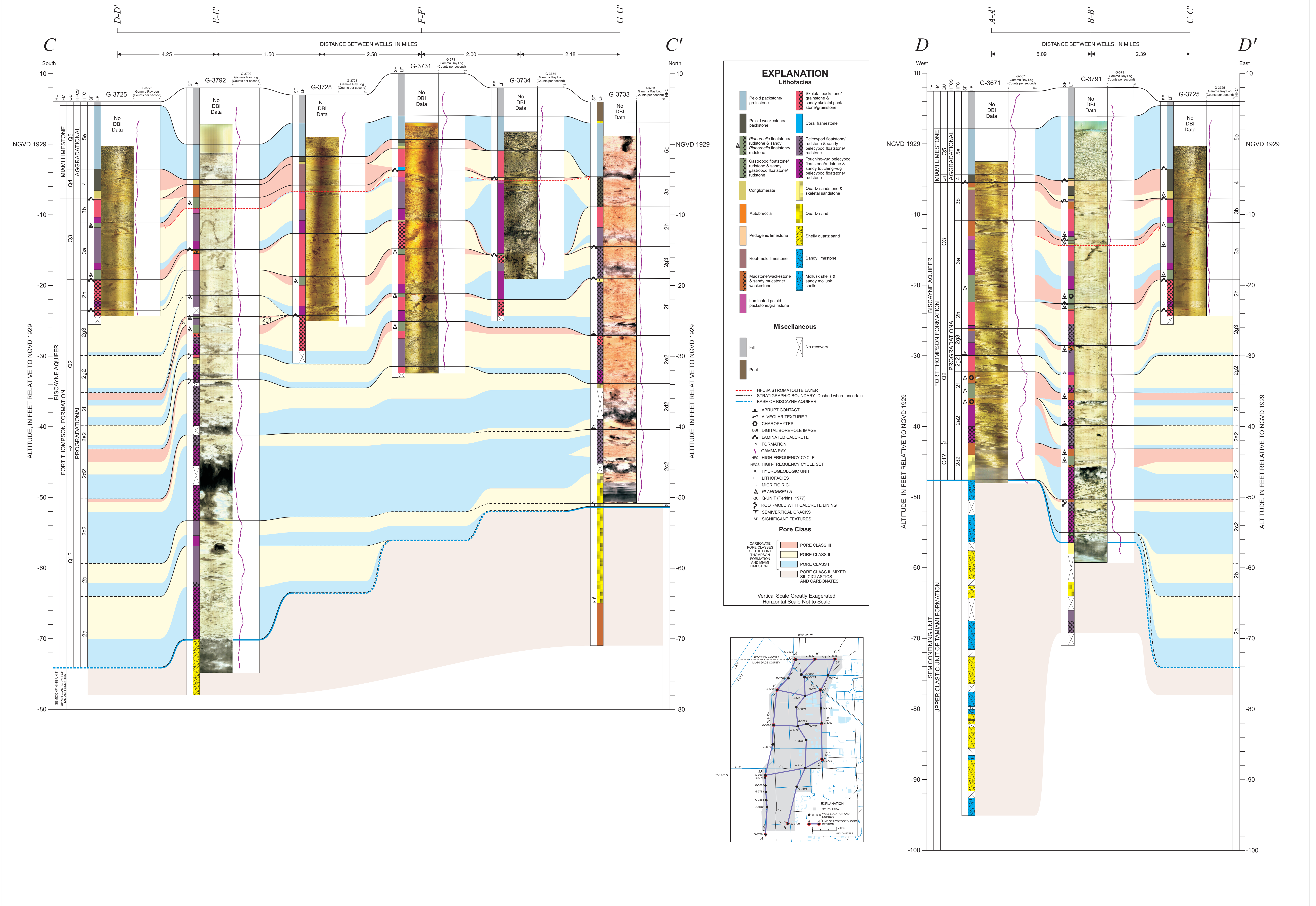
HYDROGEOLOGIC SECTIONS C-C' AND D-D' SHOWING CYCLOSTRATIGRAPHY, LITHOLOGY, AND GROUND-WATER FLOW CLASSES FOR THE BISCAYNE AQUIFER IN THE LAKE BELT AREA
