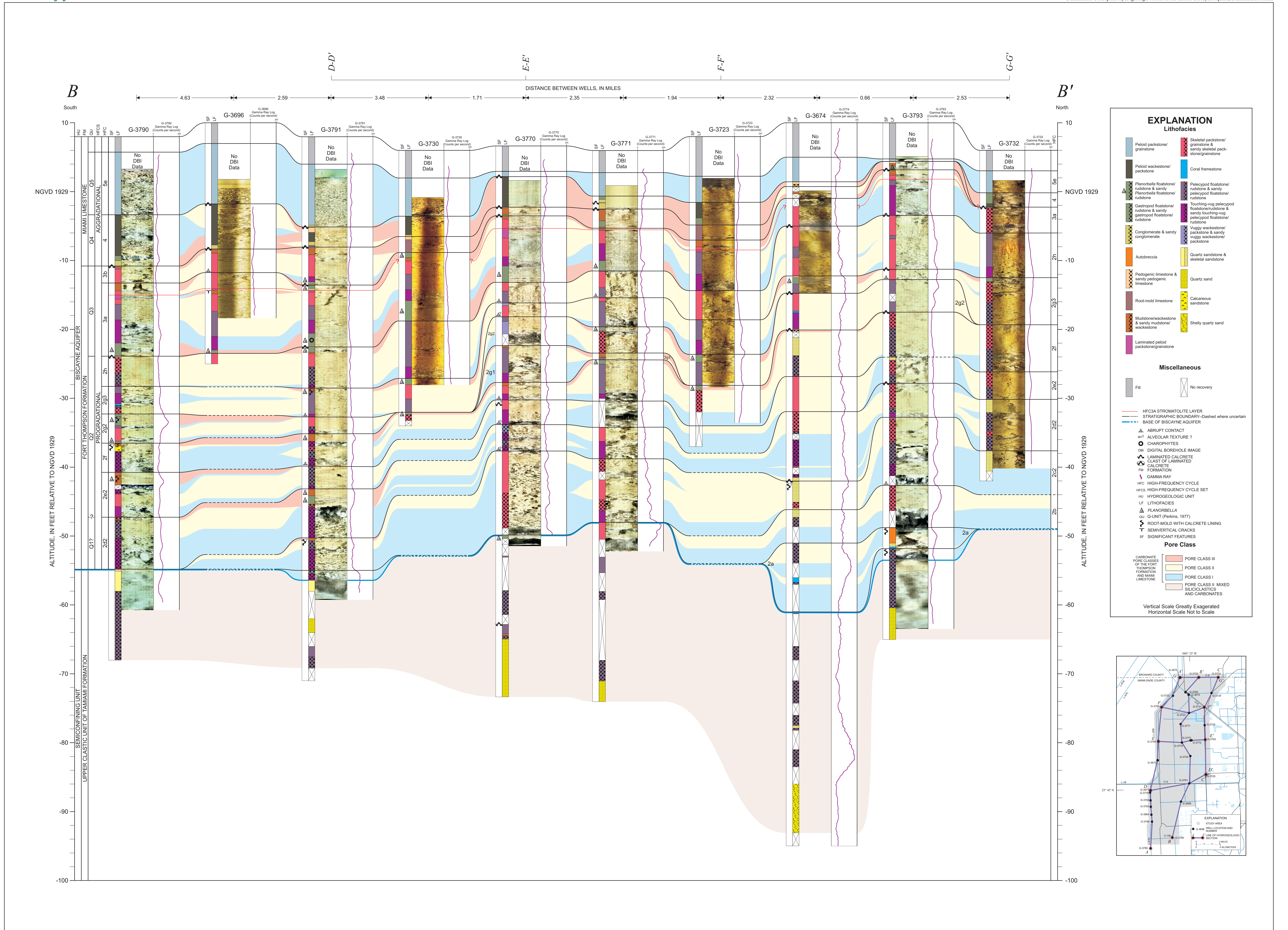
HYDROGEOLOGIC SECTION B-B' SHOWING CYCLOSTRATIGRAPHY, LITHOLOGY, AND GROUND-WATER FLOW CLASSES FOR THE BISCAYNE AQUIFER IN THE LAKE BELT AREA
