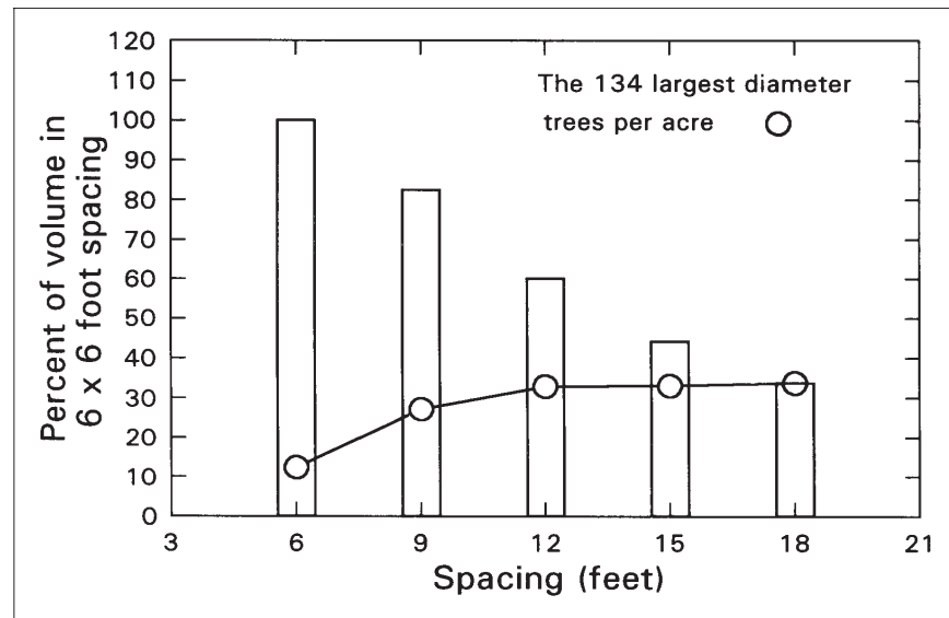
Figure 8—Percentage of 1992 total cubic volume in the narrowest spacing for each of the spacings and for the 134 largest diameter trees in each spacing. An 18-foot spacing has 134 trees per acre.
