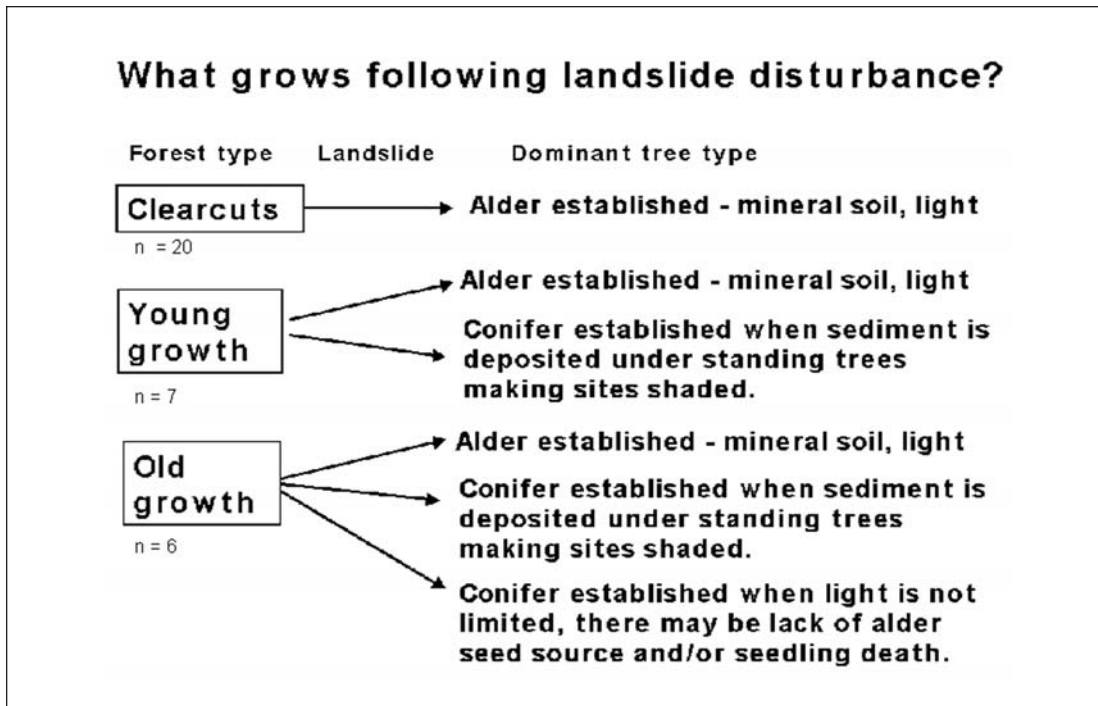
Figure 2—Pattern of alder establishment following landslide occurrence within old growth, young growth, and clearcuts.
