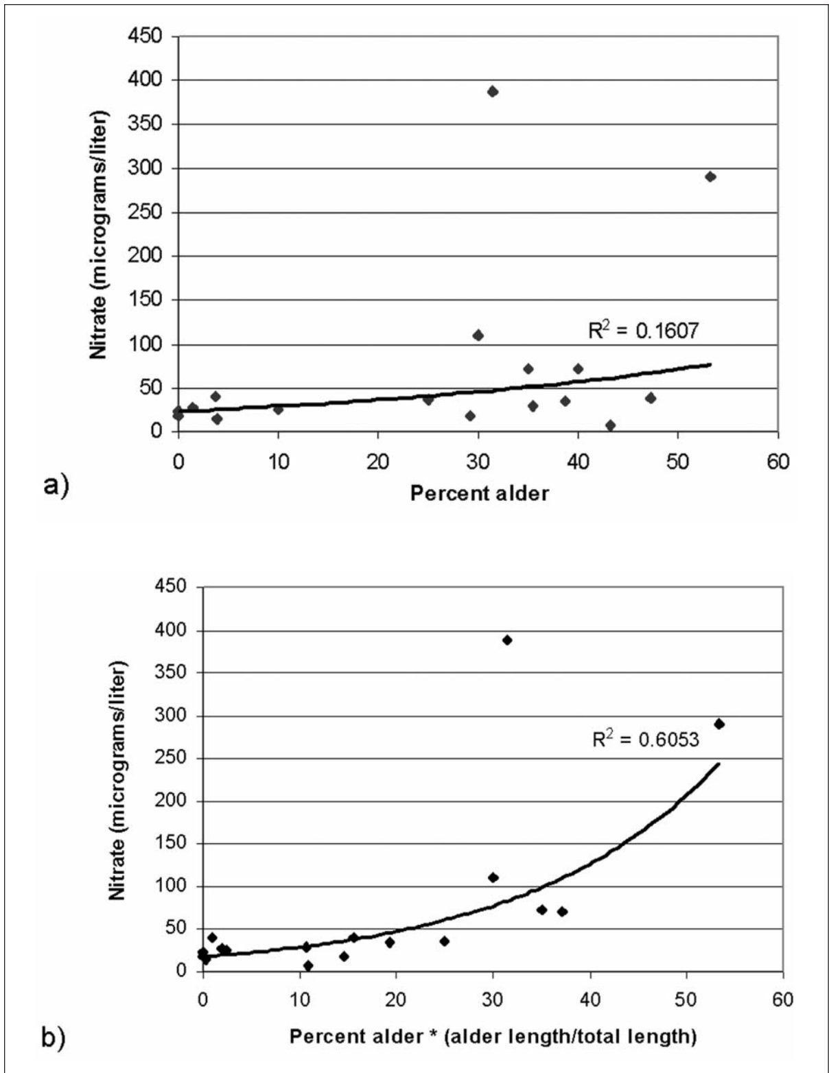
Figure 3—Relationships between nitrate concentration and a) percent alder and b) percent alder multiplied by a factor that accounts for the total length of riparian alder along selected sites.
