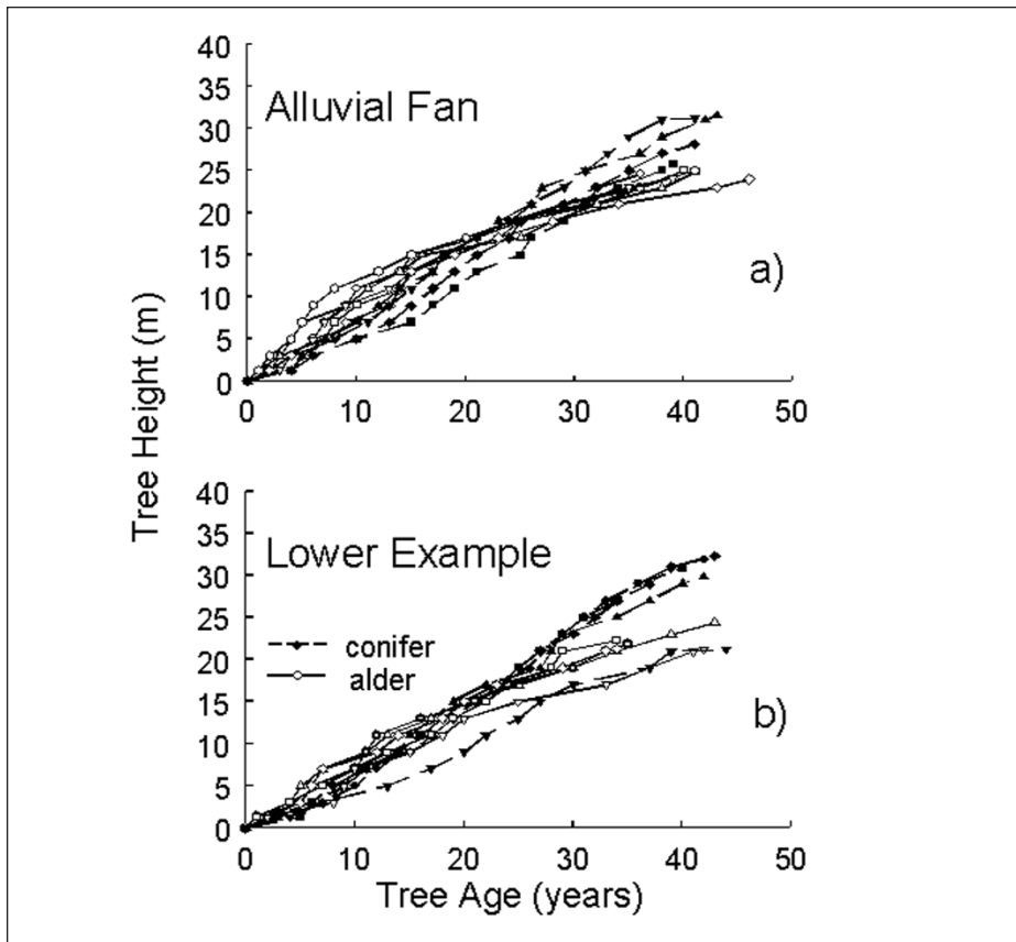
Figure 1—Tree height growth reconstructions for dominant red alders and conifers (Sitka spruce and western hemlock) at two of our research sites. The Alluvial Fan site (a) is a predominantly alder overstory stand, and the Lower Example site (b) is a conifer-dominated stand.
