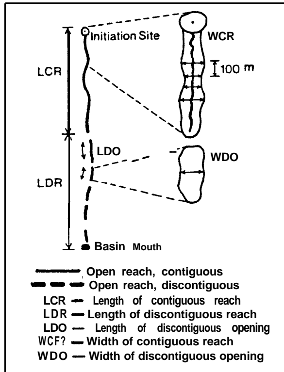
Figure 4-Measurements of length and width are made on aerial photographs of contiguous and discontinuous reaches.
