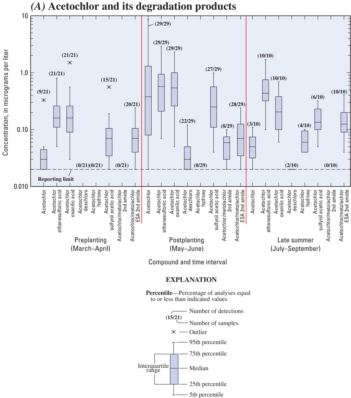
Figure 7. Concentrations of acetochlor, metolachlor, and their degradation products in water samples collected from 10 rivers in Iowa, 2004.
