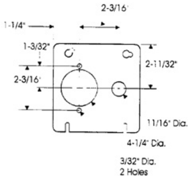
Box Cover Modification
