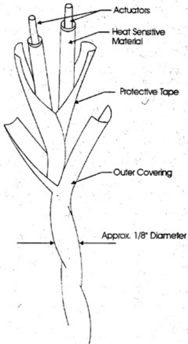
Line Heat and Fire Detector - Figure 1
