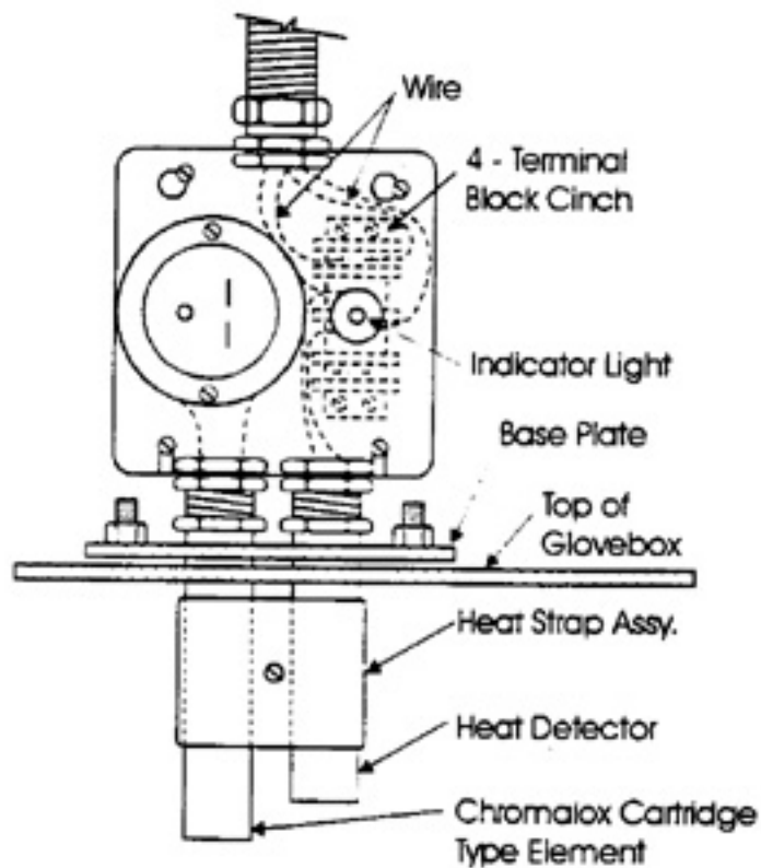
Heat Detector Assembly & Installation
