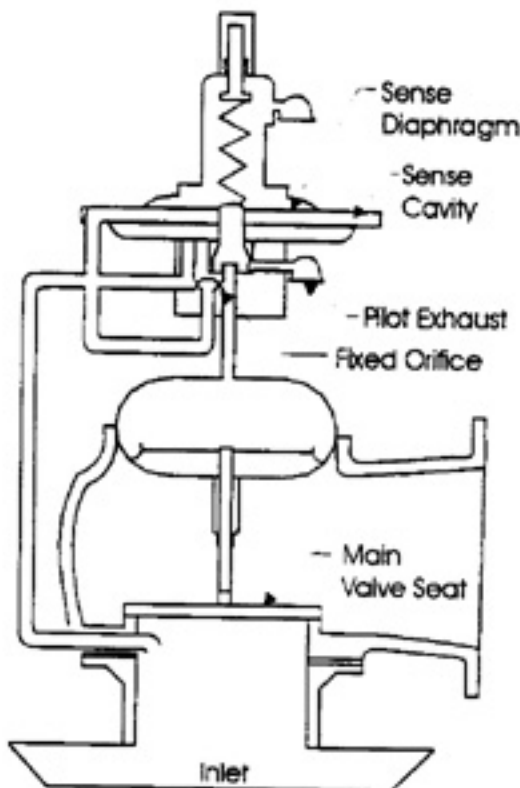
Figure 1 (Closed) Positive Pressure Relief
