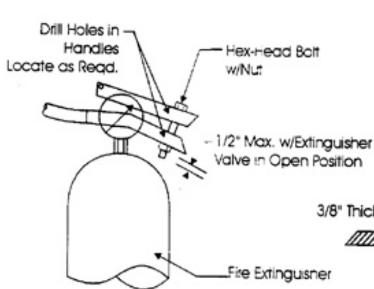
Figure 1 Elevation - Not to Scale
