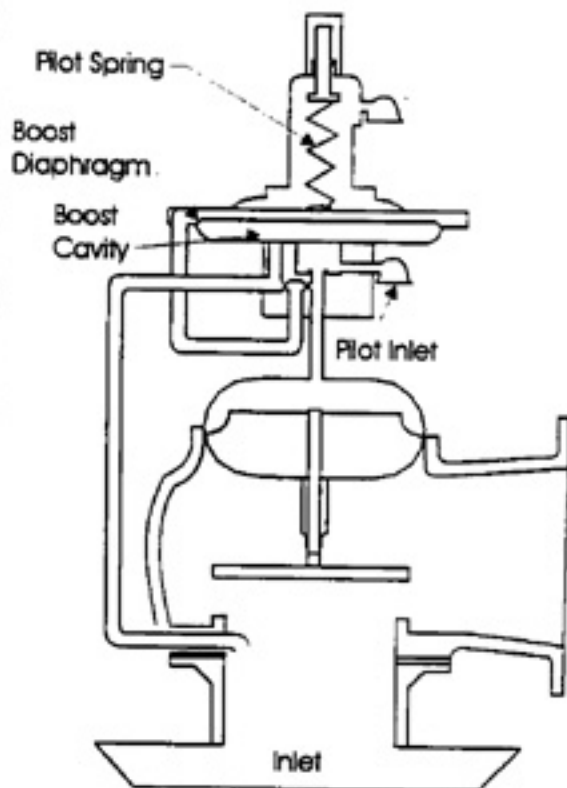
Figure 3 (Open and Flowing) Positive Pressure Relief
