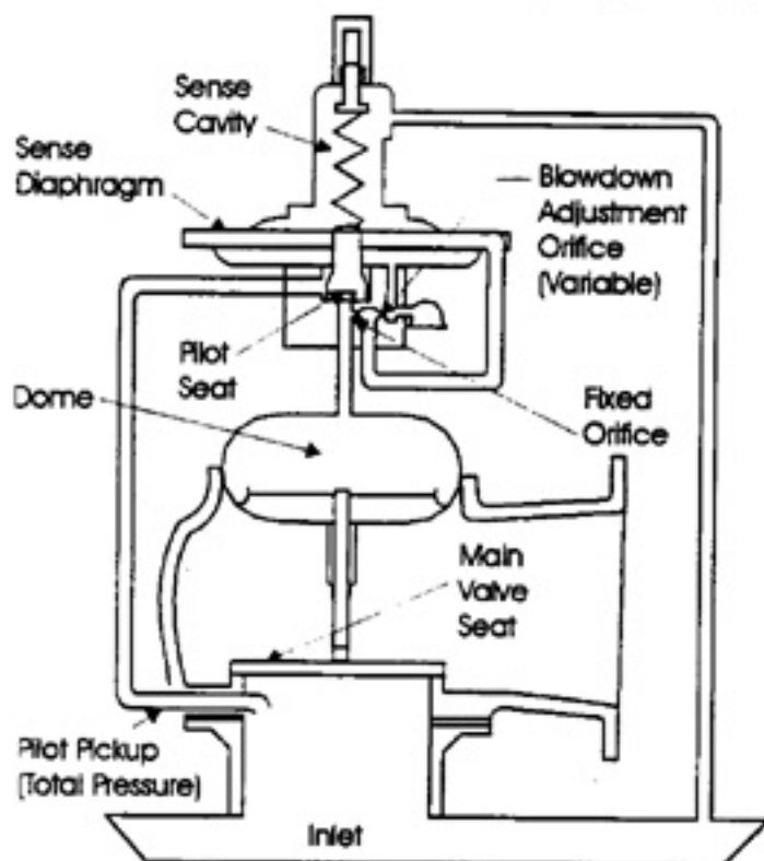
Figure 4 (Closed) Vacuum Relief
