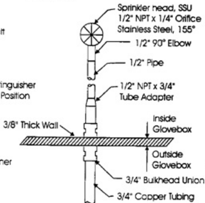
Figure 3 Plan - Not to Scale
