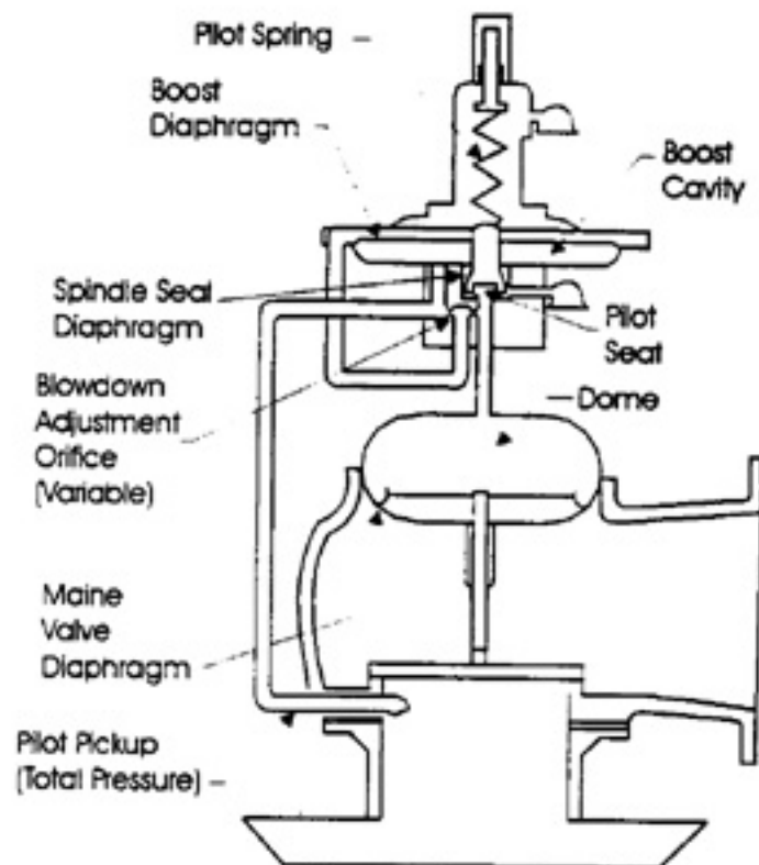
Figure 2 (Pilot Open) Positive Pressure Relief
