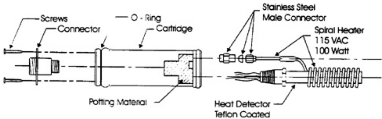
Cartridge Assembly Procedure
