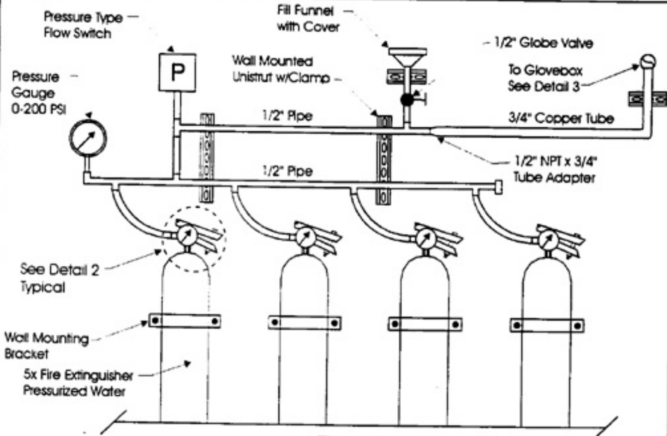
Figure 1 Elevation - Not to Scale
