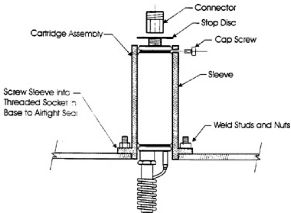
Glove Box Overheat Detector Installation Detail
