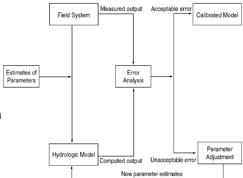
Figure 4. Calibration procedure of hydrological models.
