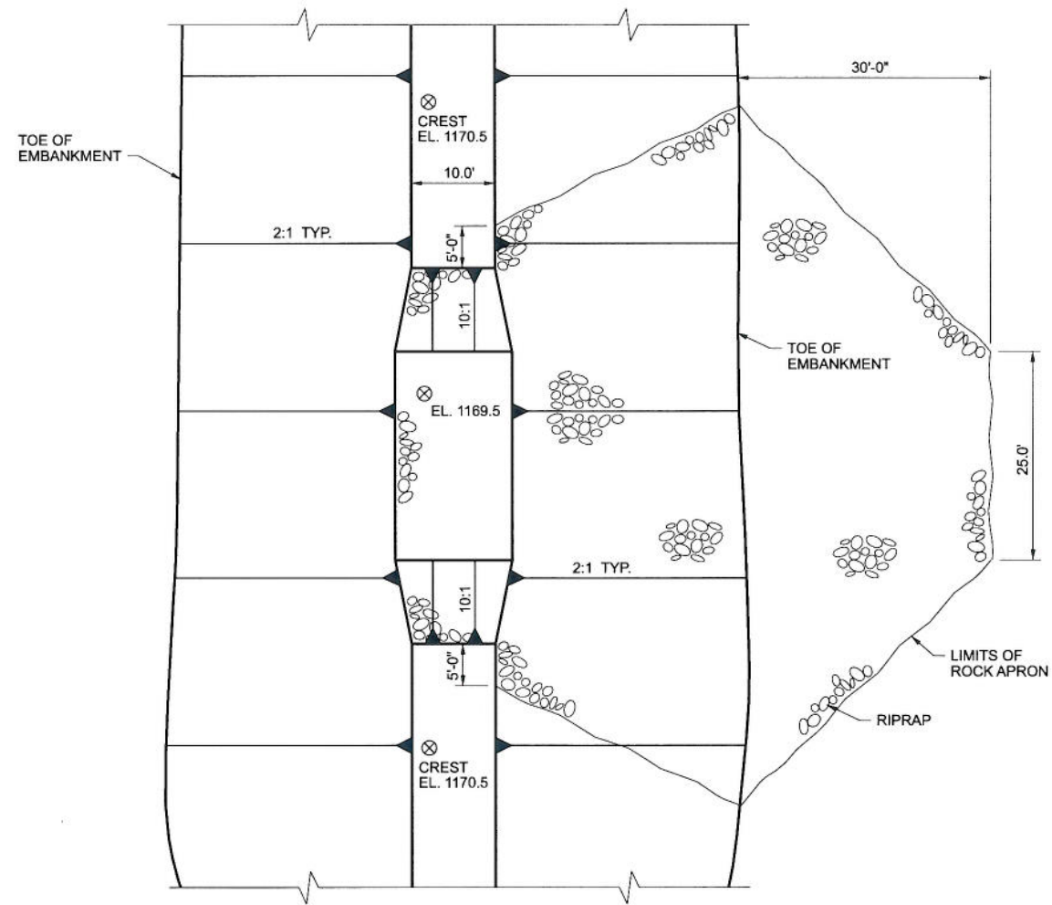
ROCK APRON OVERFLOW DETAIL 1/2"=1'-0"
