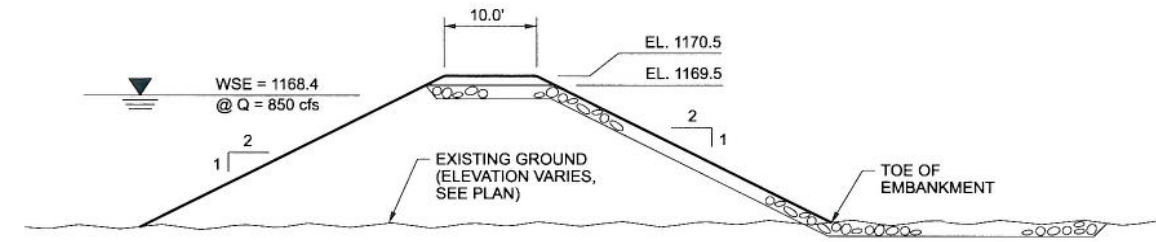
TYPICAL SECTION 1/2"=1'-0"
