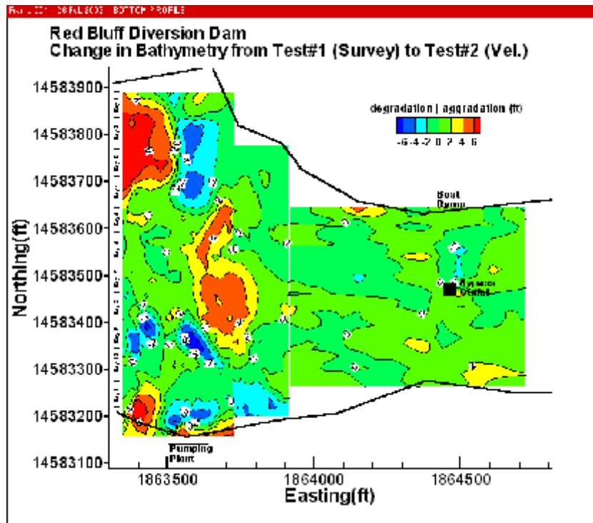
Figure 11 - Change in river bathymetry from test 1 to test 2.
